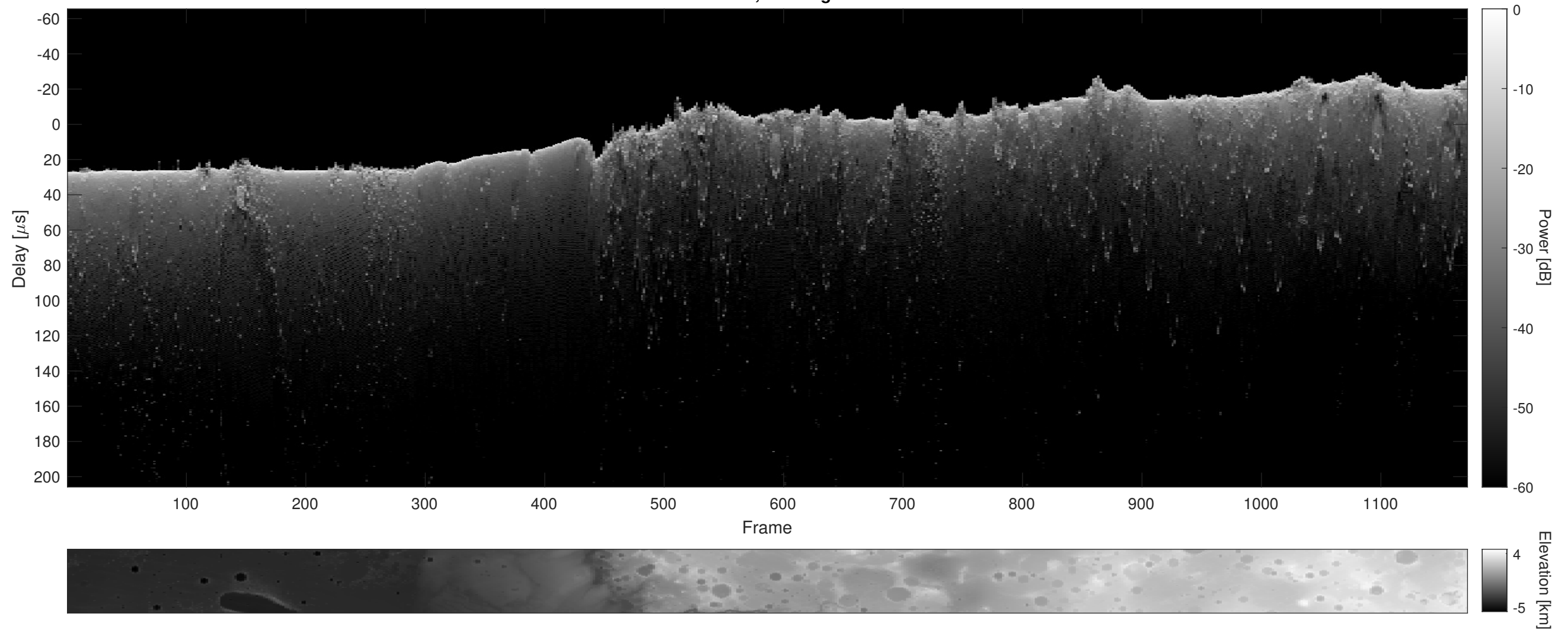
Orbit 9134, Cluttergram
