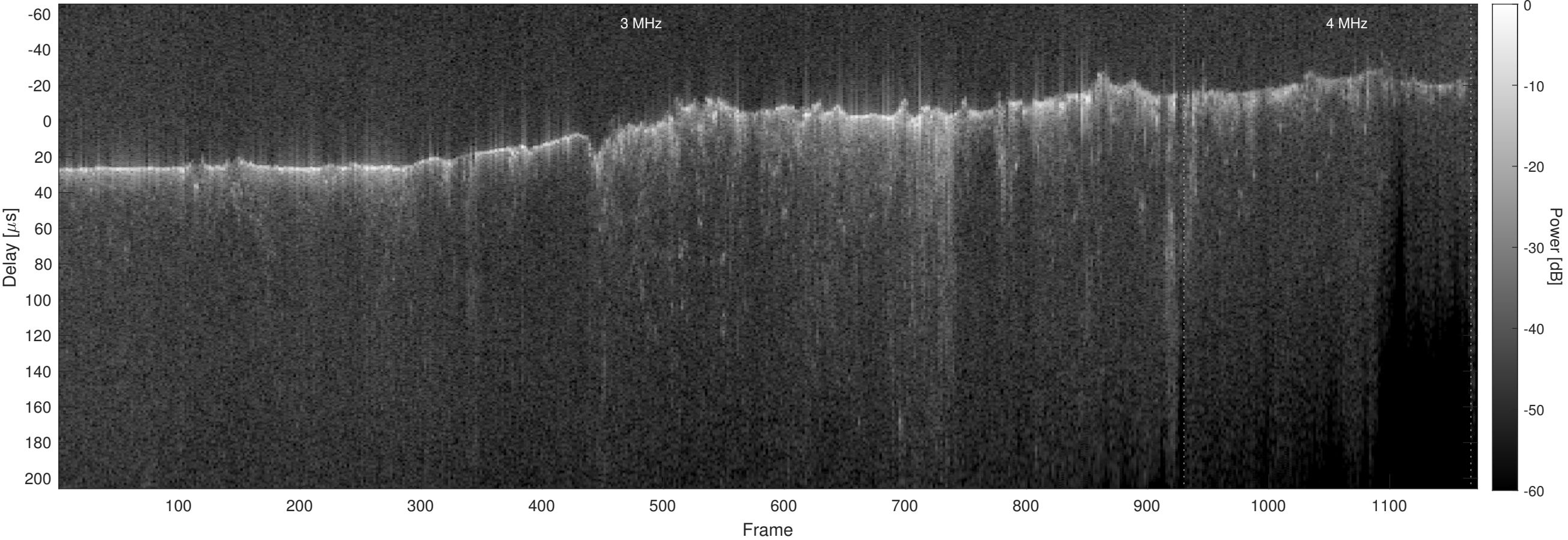
Orbit 9134, Optimized, No Window, Channel 2
