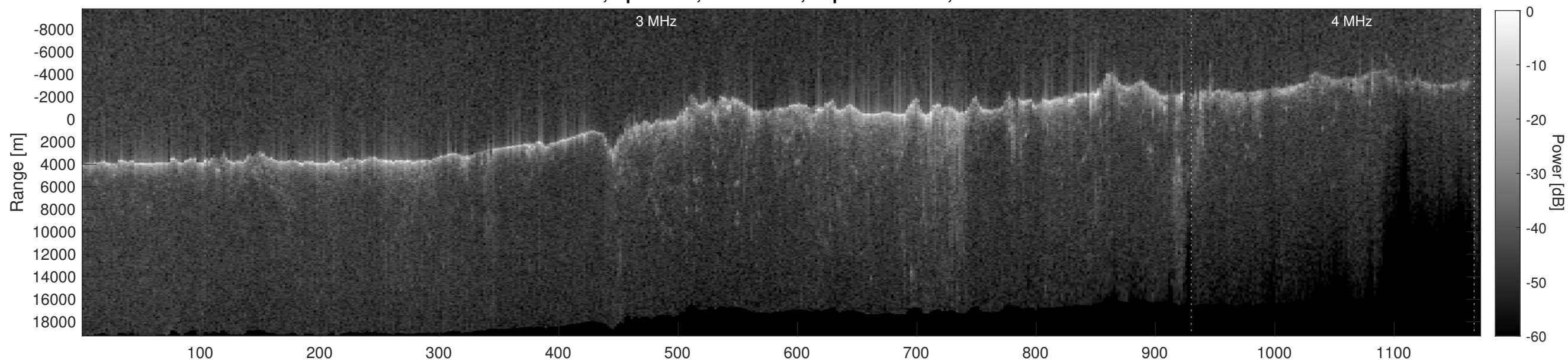
Orbit 9134, Depth-Corrected Cluttergram
