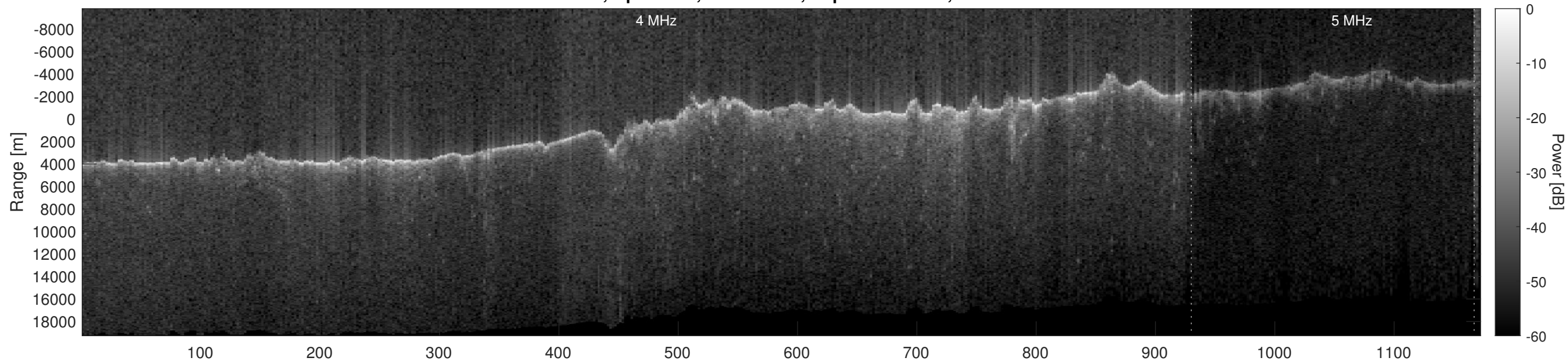
Orbit 9134, Optimized, No Window, Depth-Corrected, Channel 2
