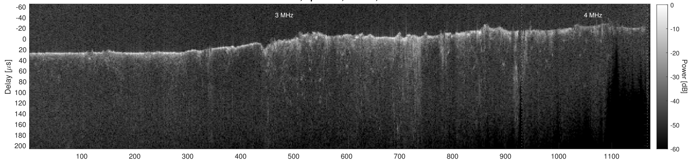
Orbit 9134, Cluttergram
