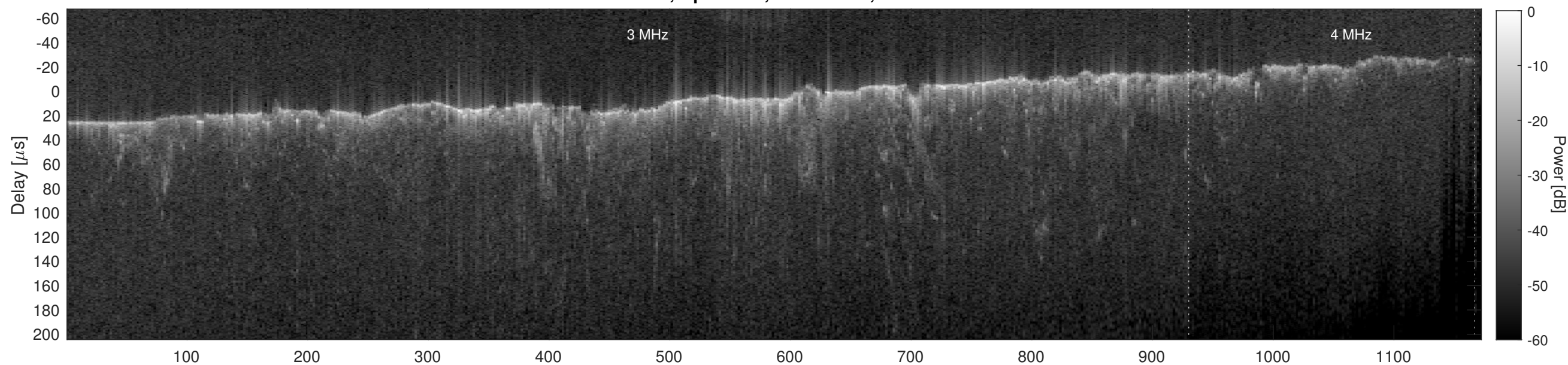
Orbit 9136, Cluttergram
