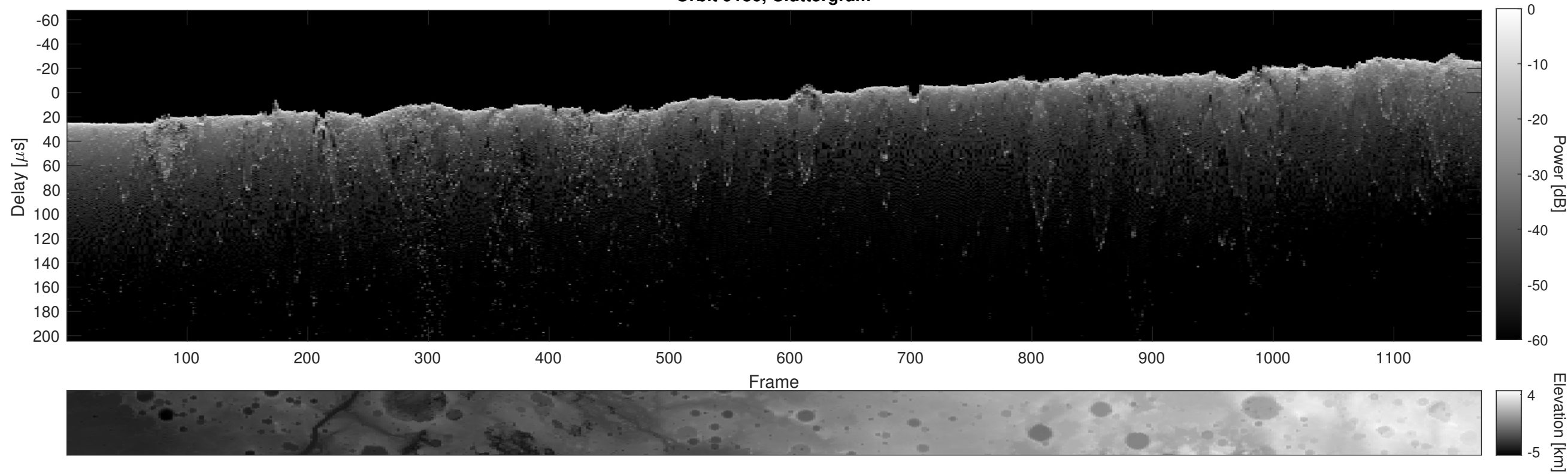
Orbit 9136, Cluttergram
