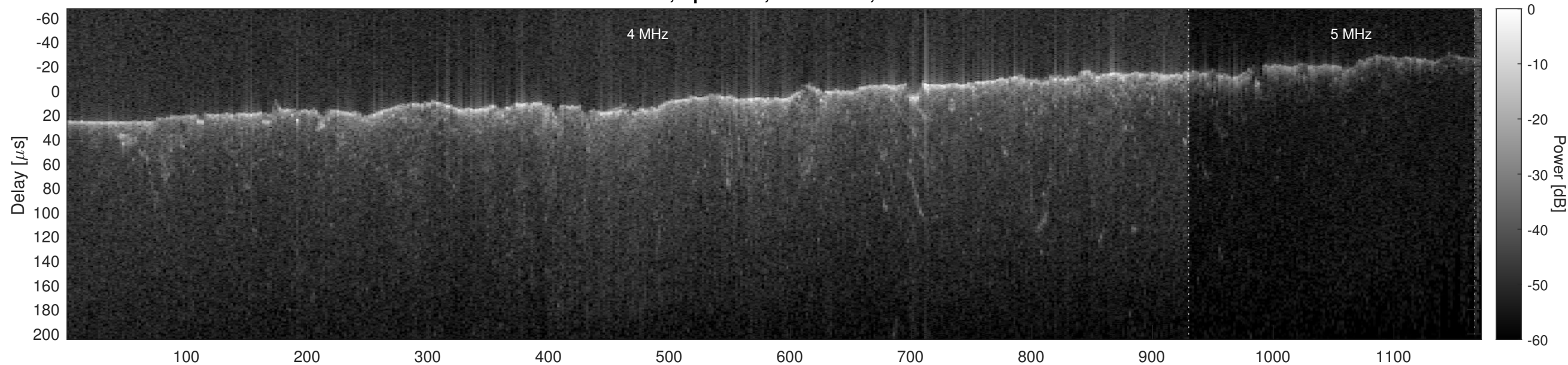
Orbit 9136, Optimized, No Window, Channel 2
