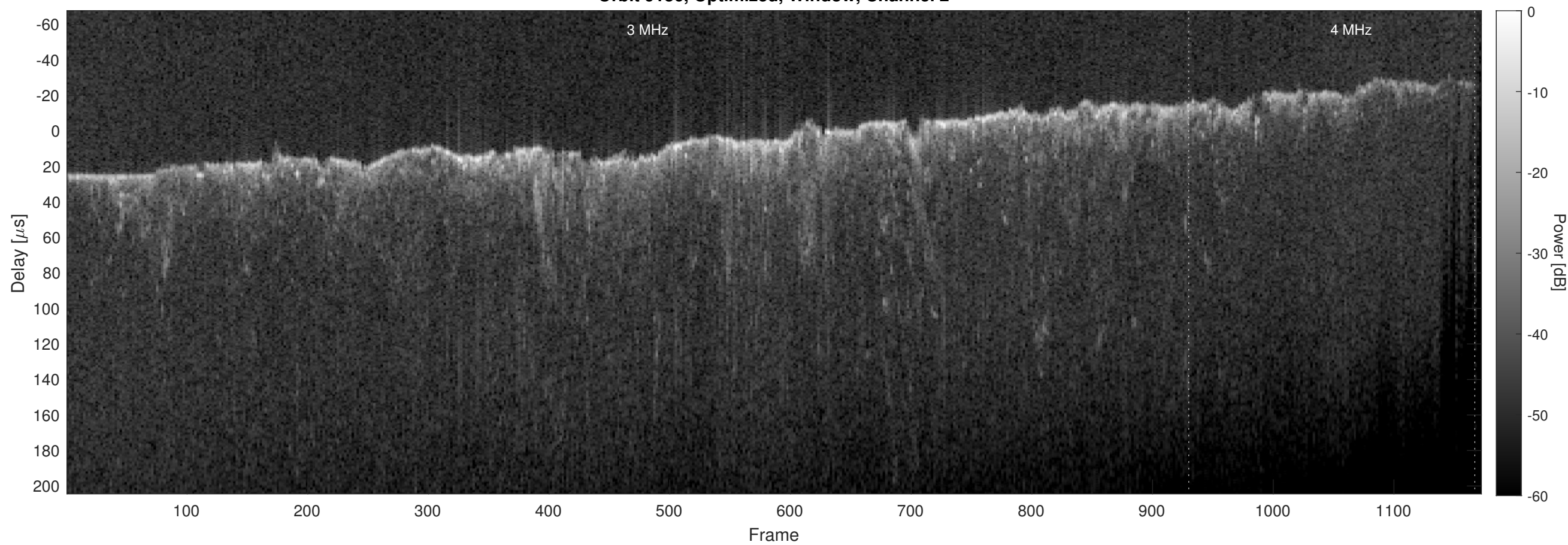
Orbit 9136, Optimized, Window, Channel 2
