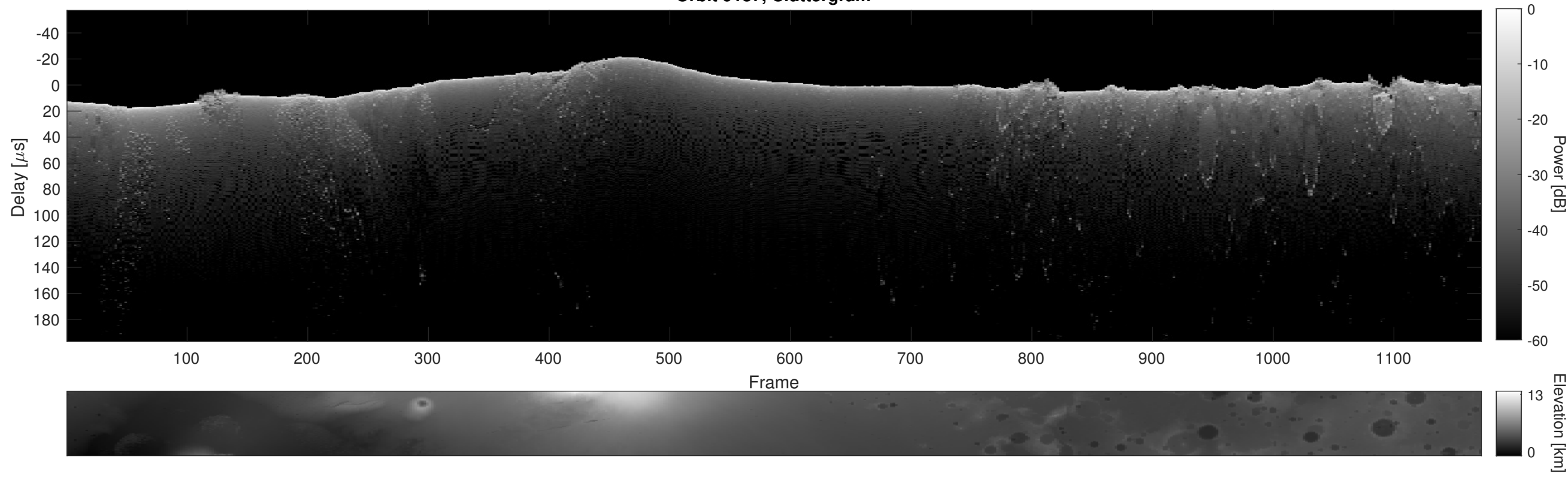
Orbit 9137, Cluttergram
