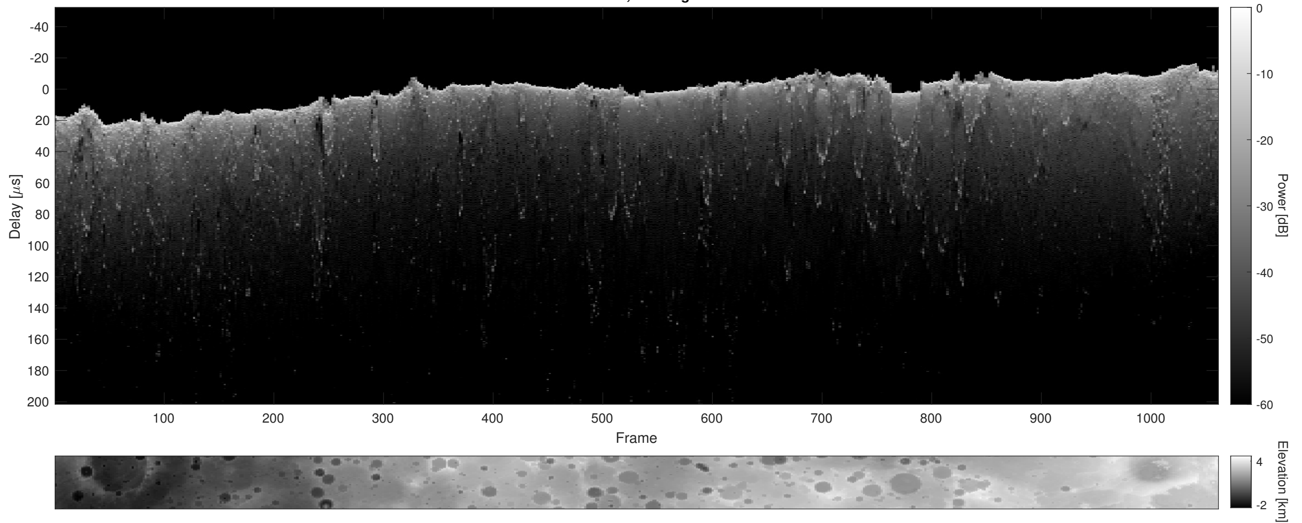
Orbit 9139, Cluttergram
