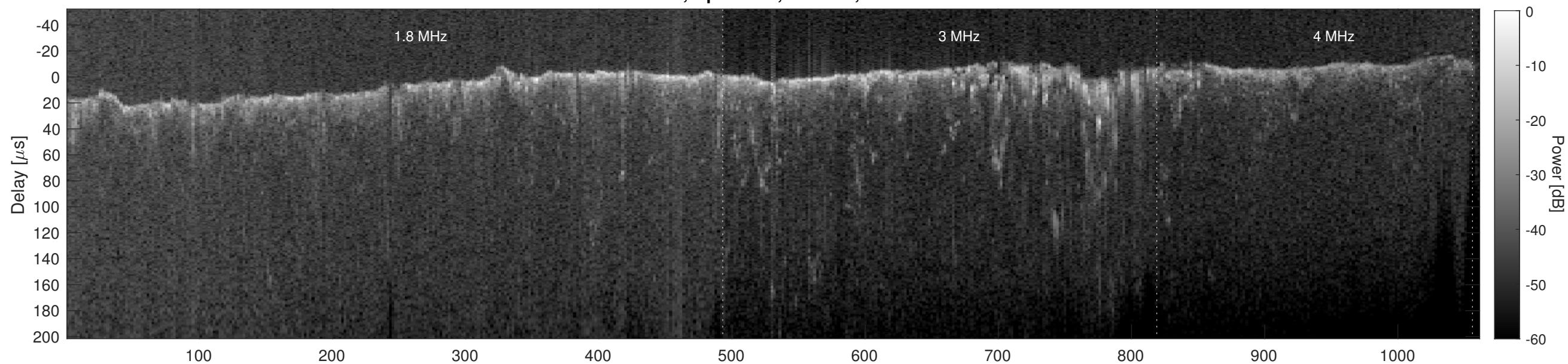
Orbit 9139, Cluttergram
