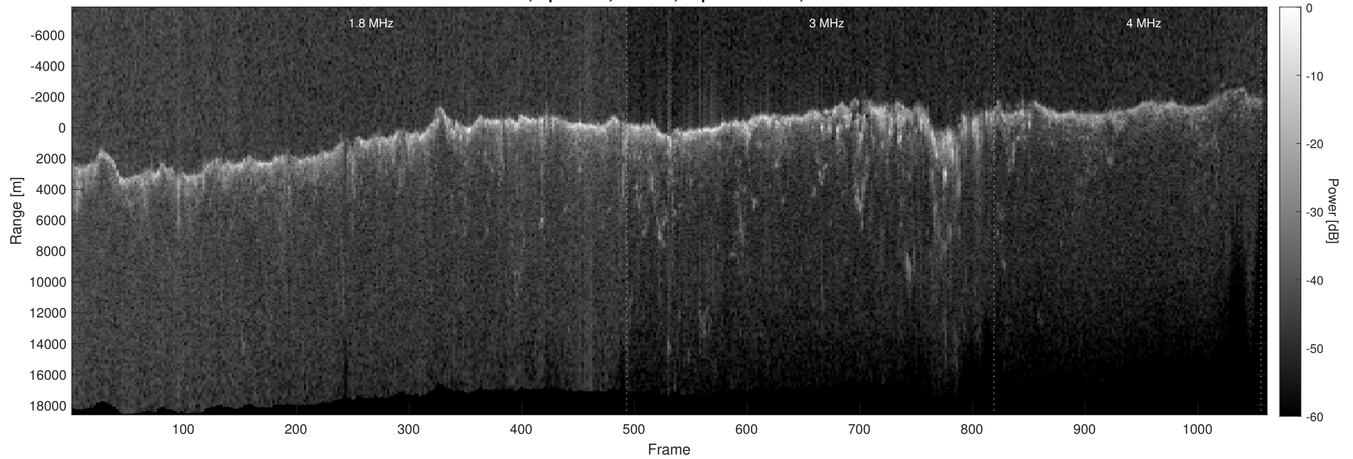
Orbit 9139, Optimized, Window, Depth-Corrected, Channel 2
