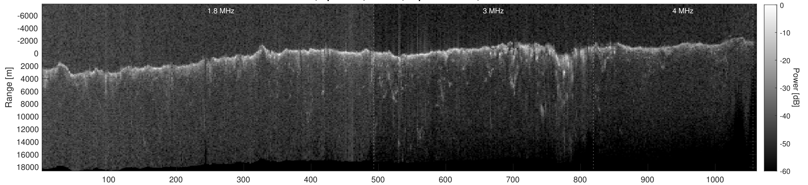
Orbit 9139, Depth-Corrected Cluttergram
