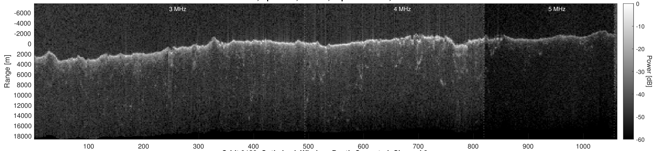
Orbit 9139, Optimized, Window, Depth-Corrected, Channel 2
