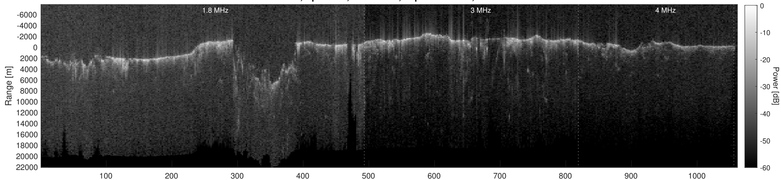
Orbit 9140, Depth-Corrected Cluttergram
