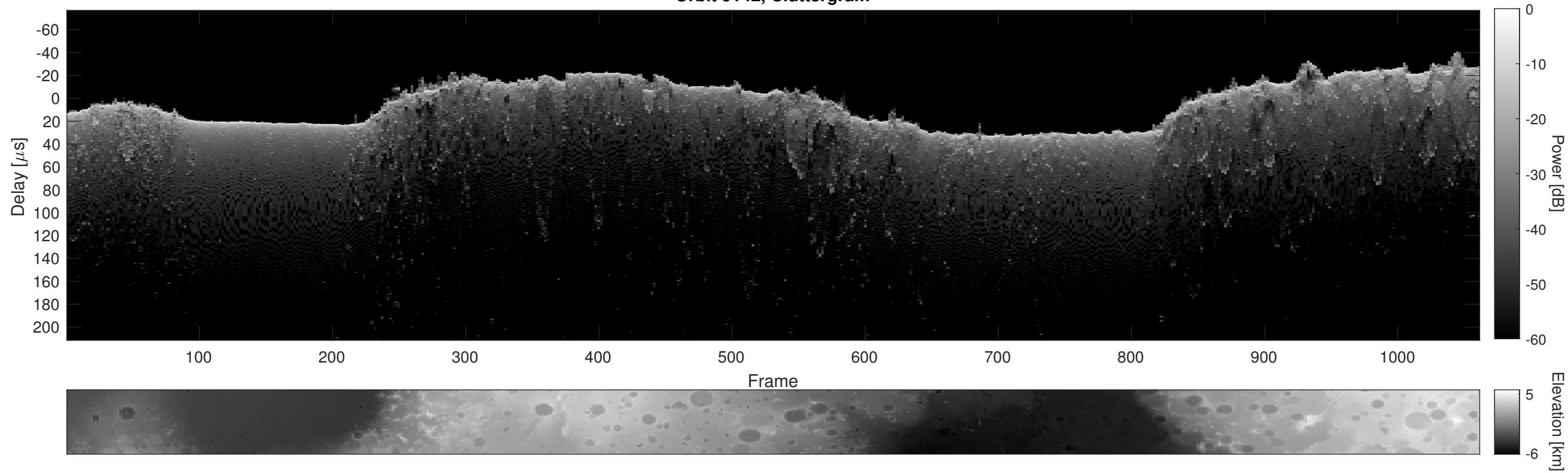
Orbit 9142, Cluttergram
