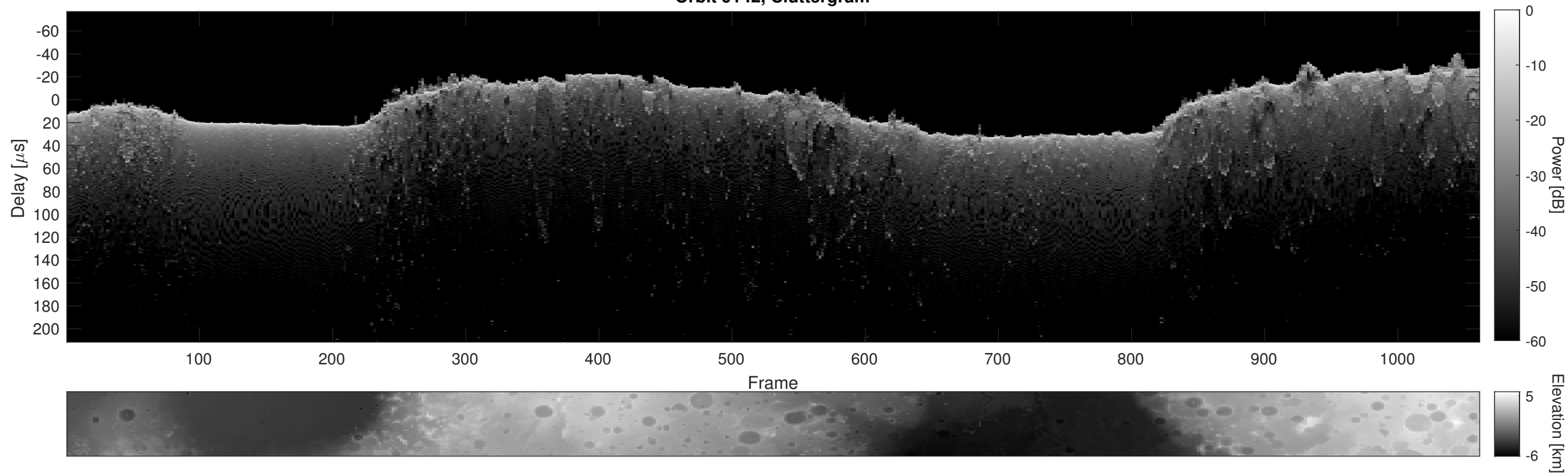
Orbit 9142, Cluttergram
