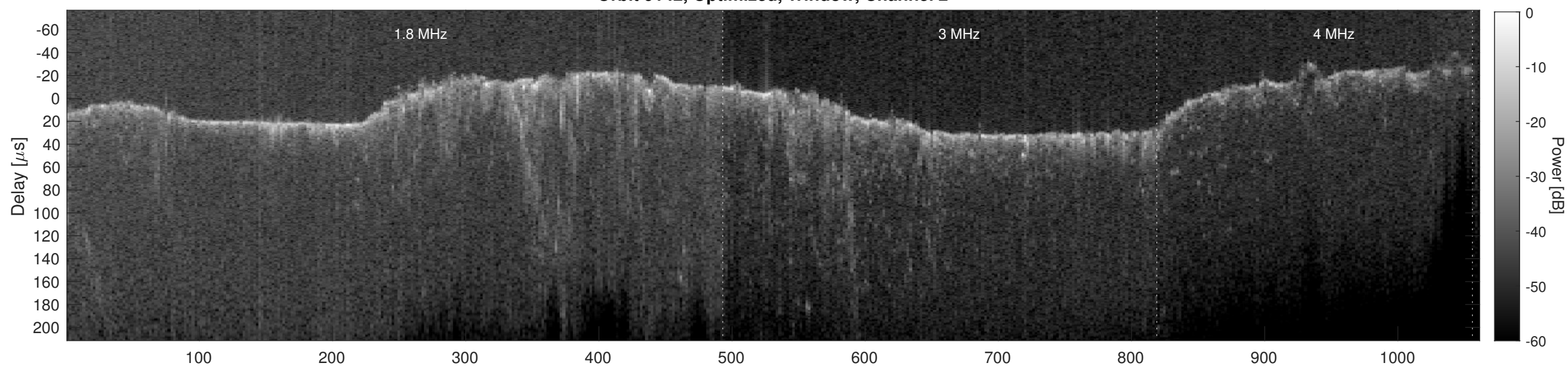
Orbit 9142, Cluttergram
