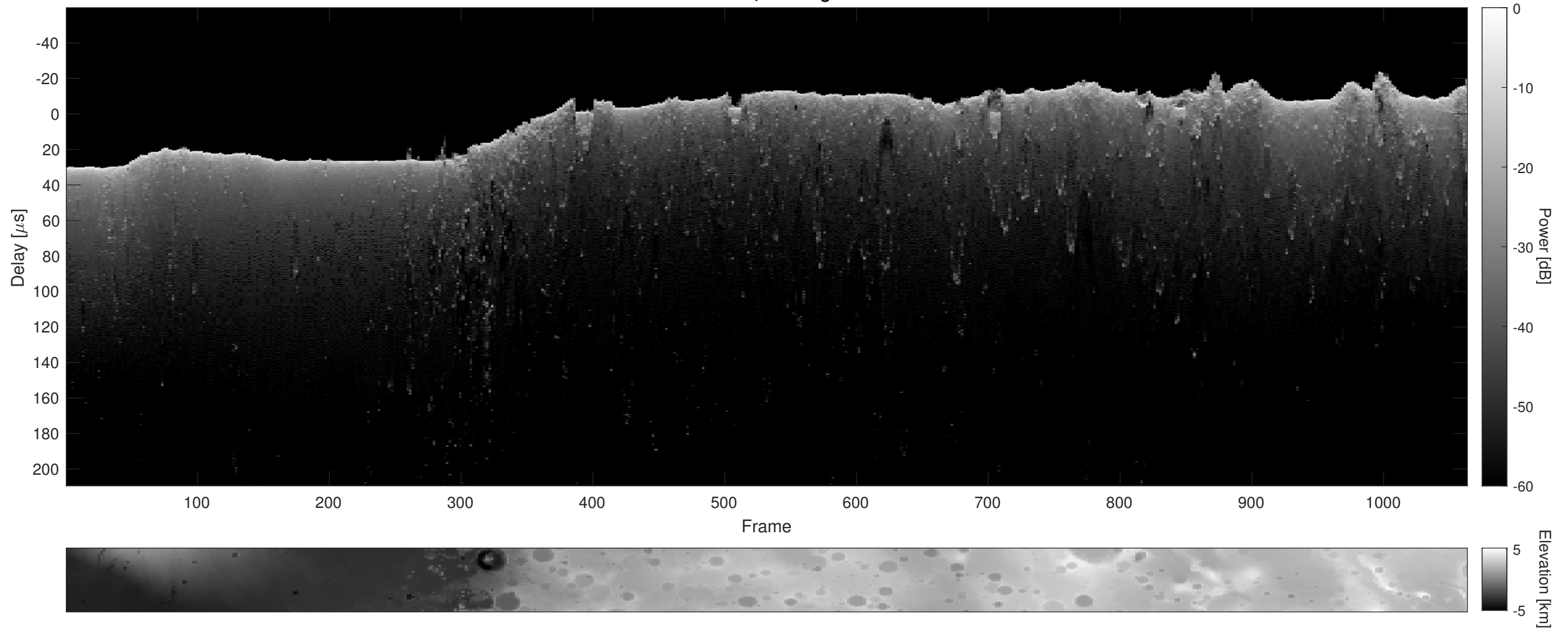
Orbit 9145, Cluttergram
