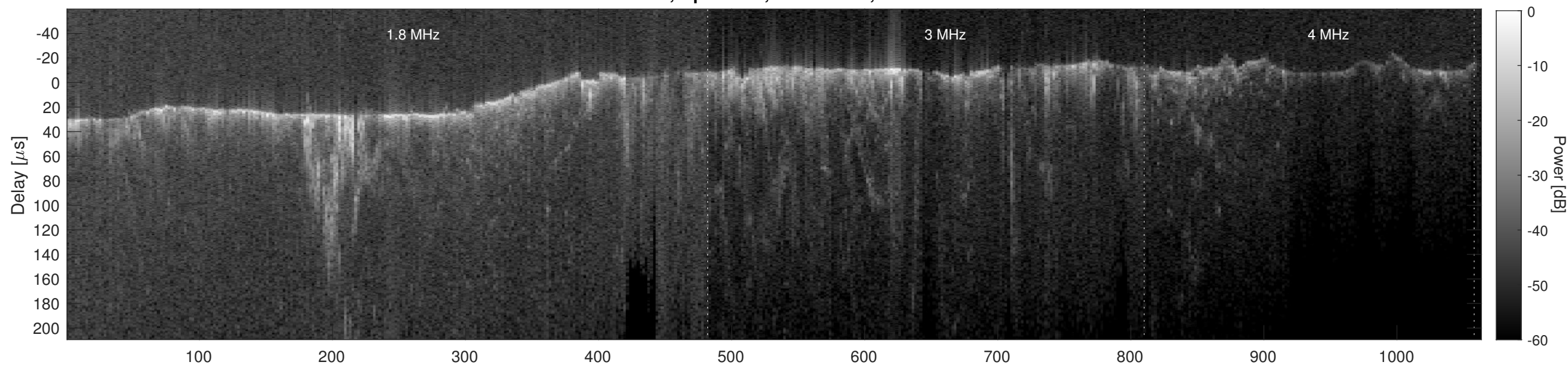
Orbit 9145, Cluttergram
