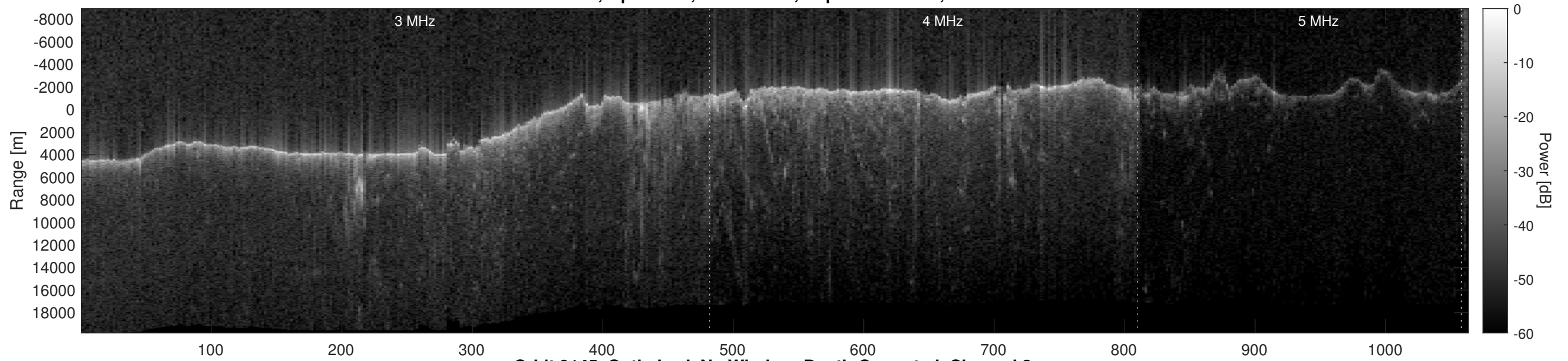
Orbit 9145, Optimized, No Window, Depth-Corrected, Channel 2
