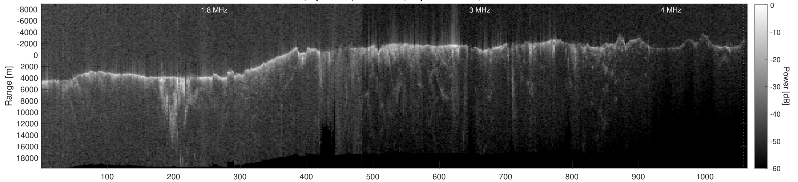
Orbit 9145, Depth-Corrected Cluttergram
