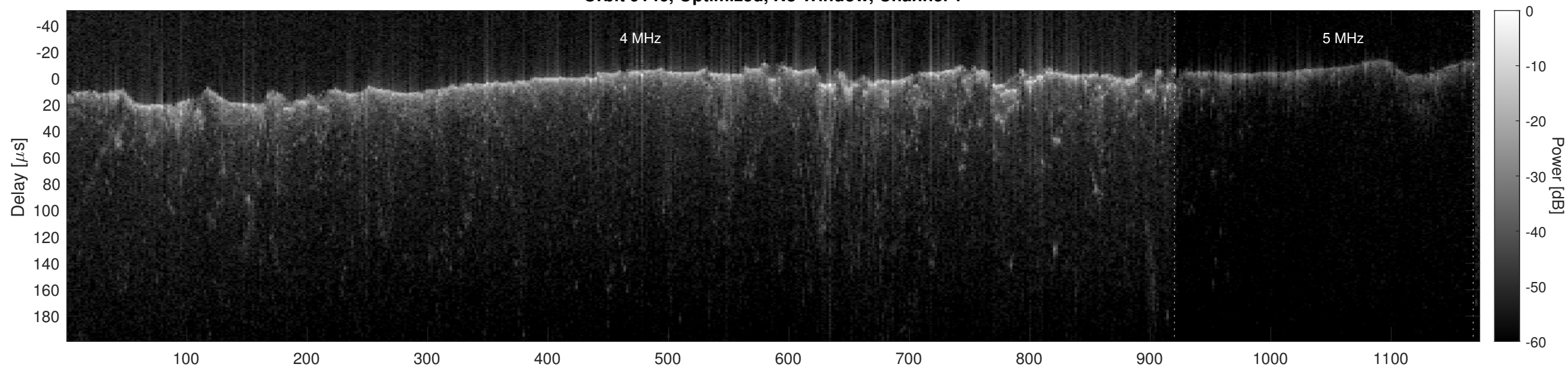
Orbit 9146, Optimized, No Window, Channel 2
