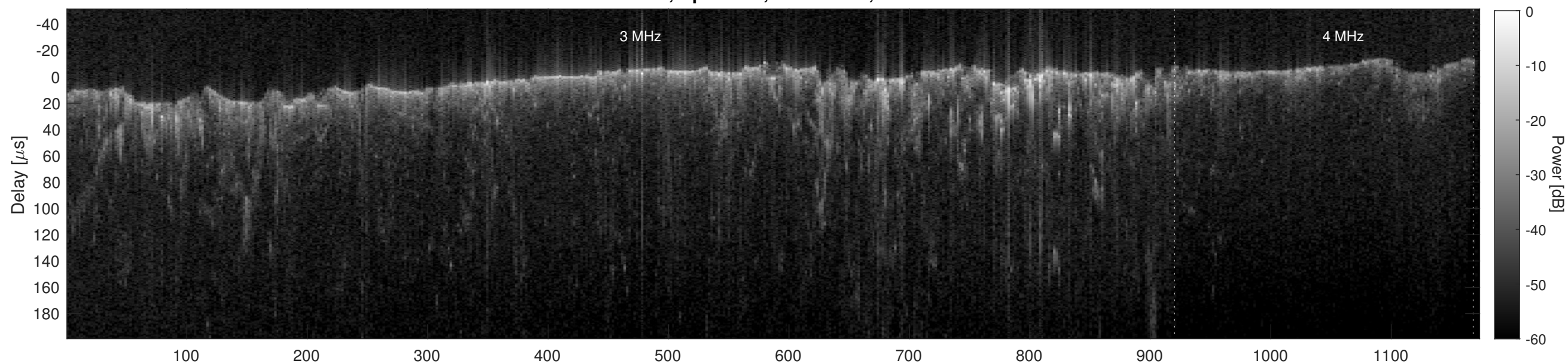
Orbit 9146, Cluttergram
