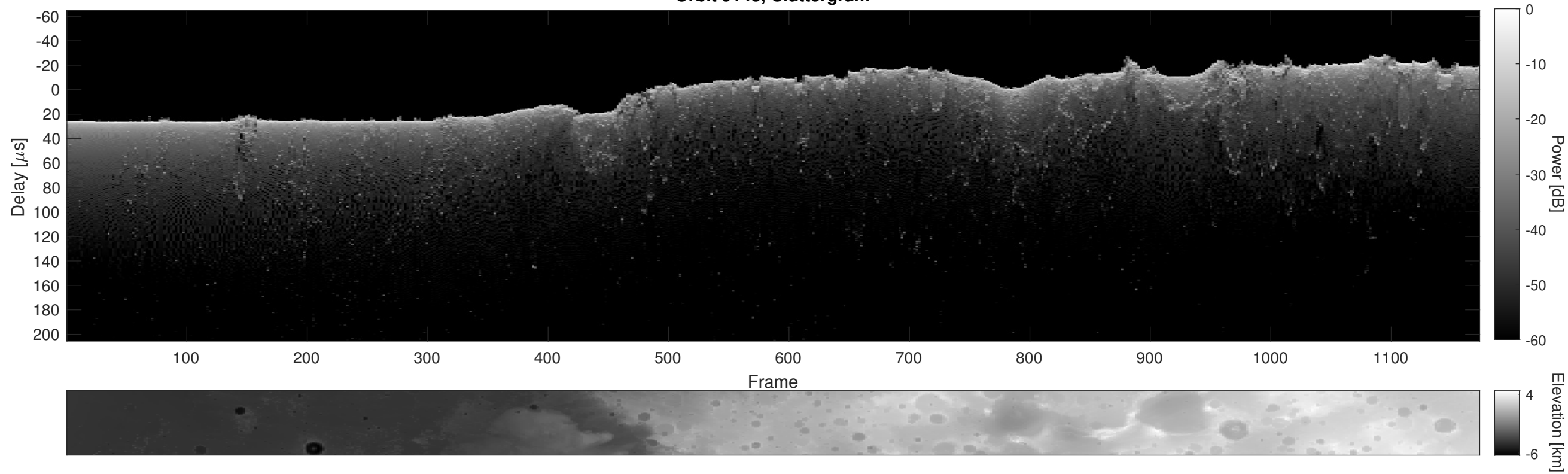
Orbit 9148, Cluttergram
