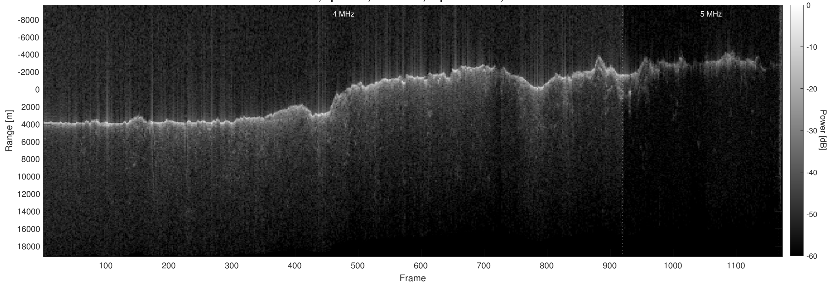
Orbit 9148, Optimized, No Window, Depth-Corrected, Channel 2
