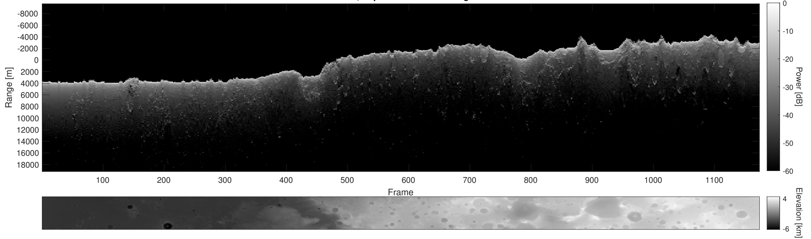
Orbit 9148, Depth-Corrected Cluttergram
