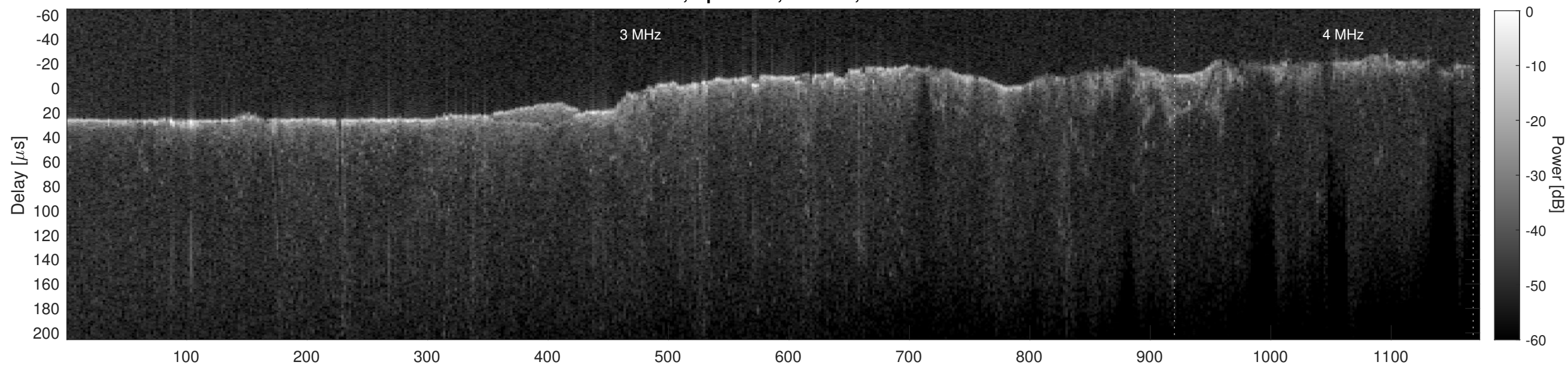
Orbit 9148, Cluttergram
