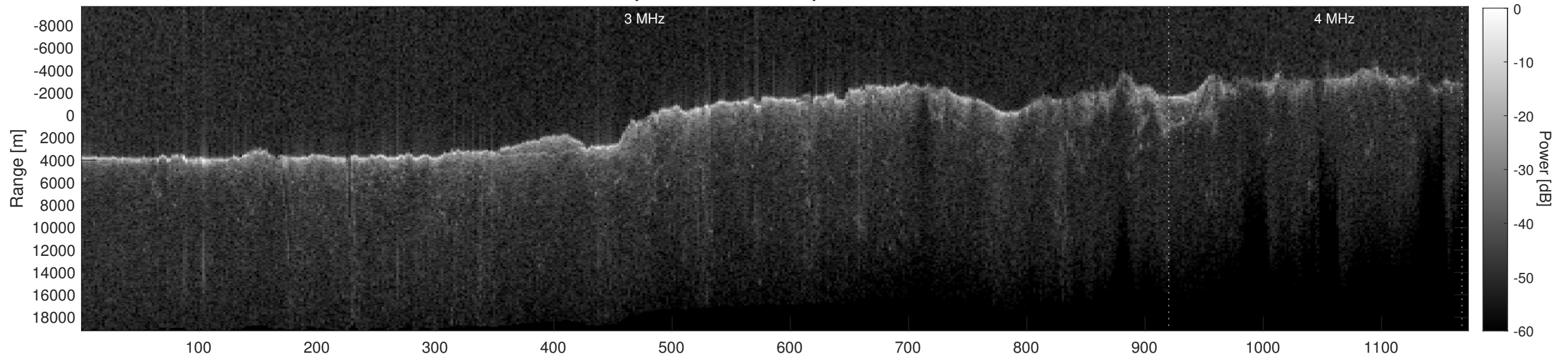
Orbit 9148, Depth-Corrected Cluttergram
