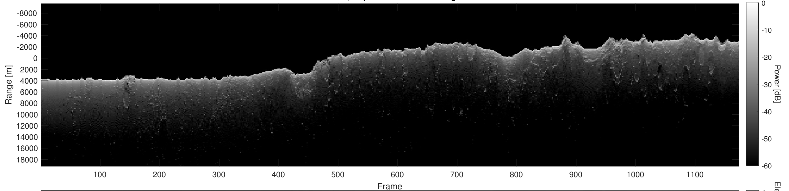
Orbit 9148, Depth-Corrected Cluttergram
