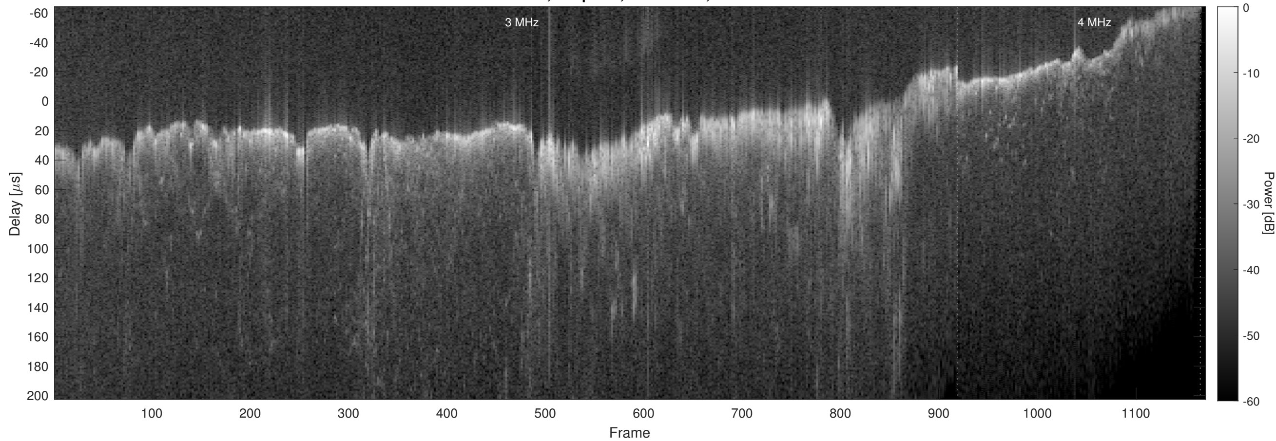
Orbit 9150, Chapman, No Window, Channel 2
