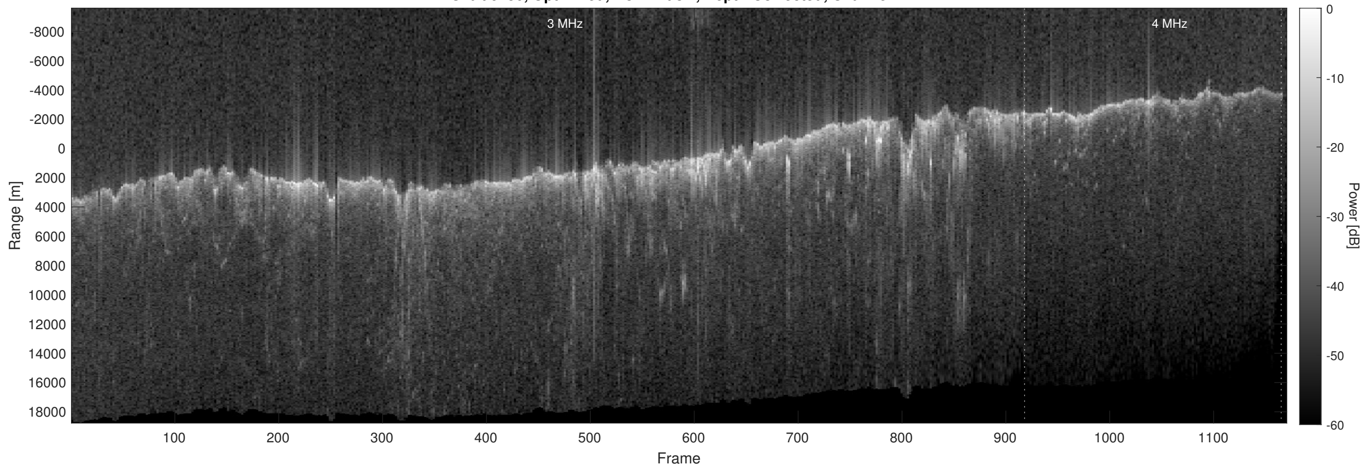
Orbit 9150, Optimized, No Window, Depth-Corrected, Channel 2
