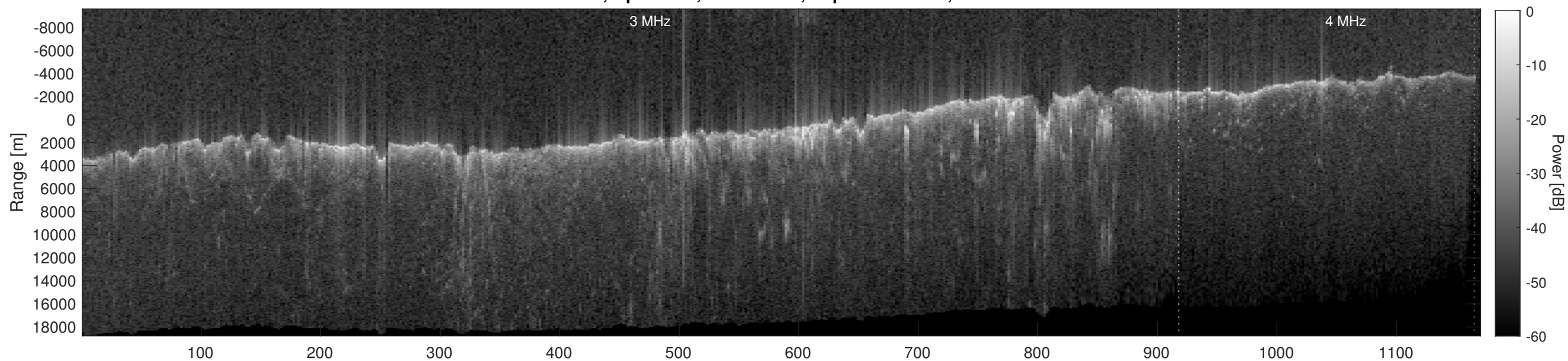
Orbit 9150, Depth-Corrected Cluttergram
