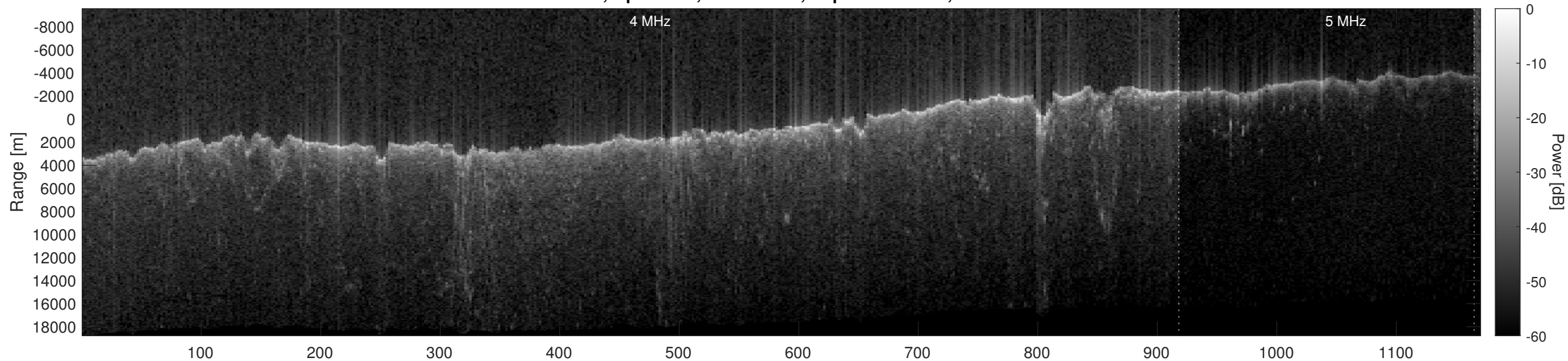
Orbit 9150, Optimized, No Window, Depth-Corrected, Channel 2
