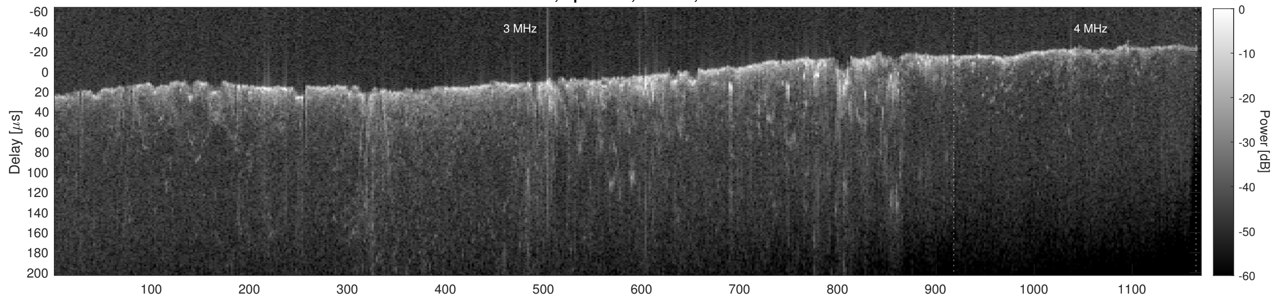
Orbit 9150, Cluttergram
