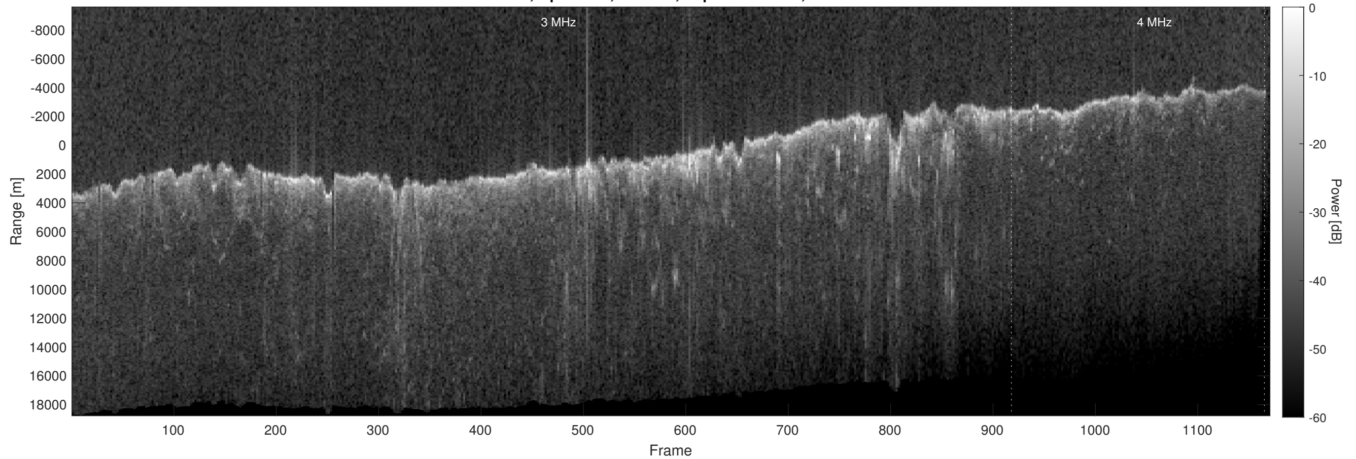
Orbit 9150, Optimized, Window, Depth-Corrected, Channel 2
