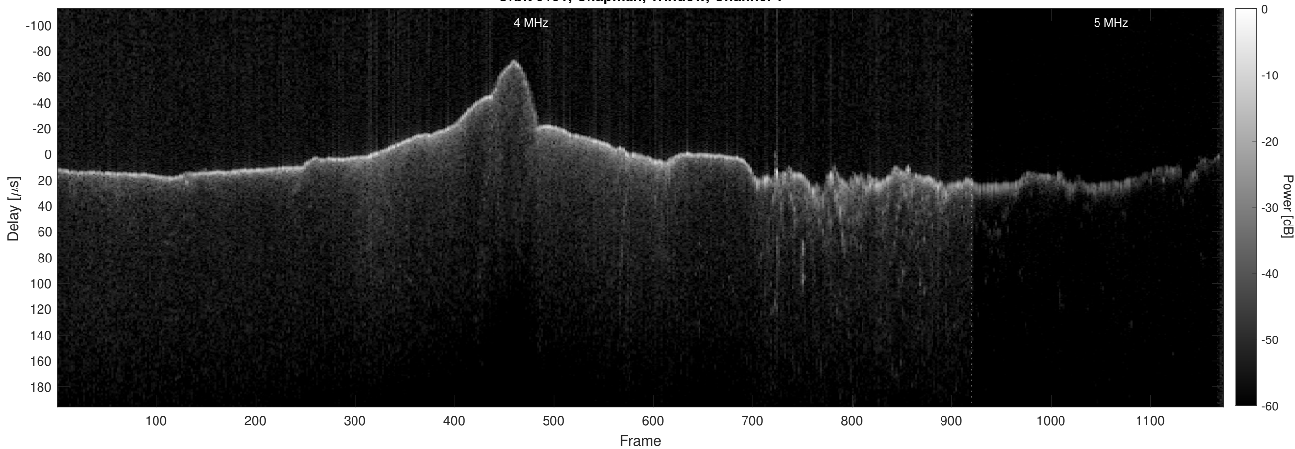
Orbit 9151, Chapman, Window, Channel 2
