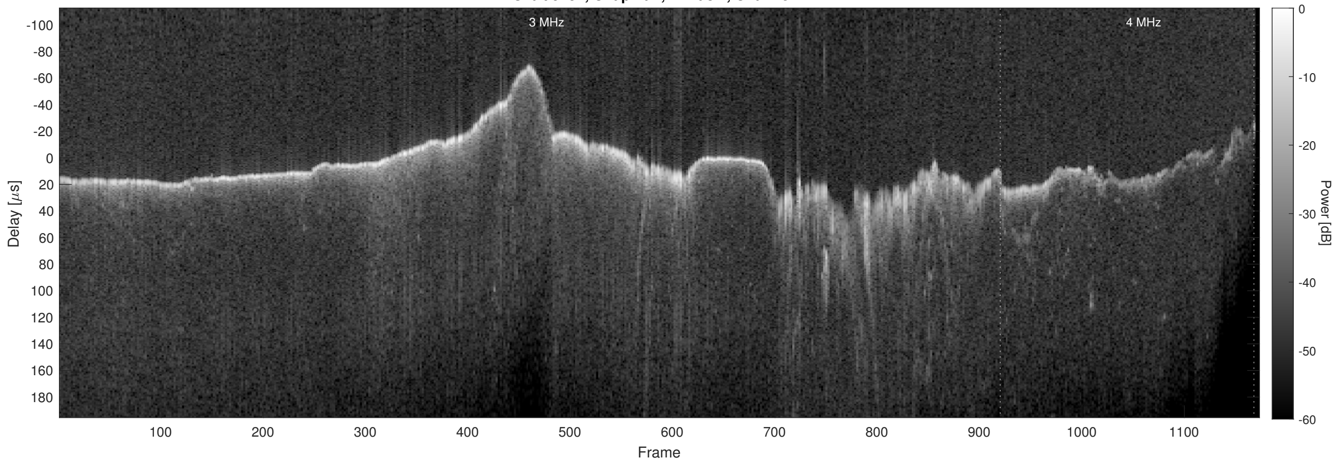
Orbit 9151, Chapman, Window, Channel 2
