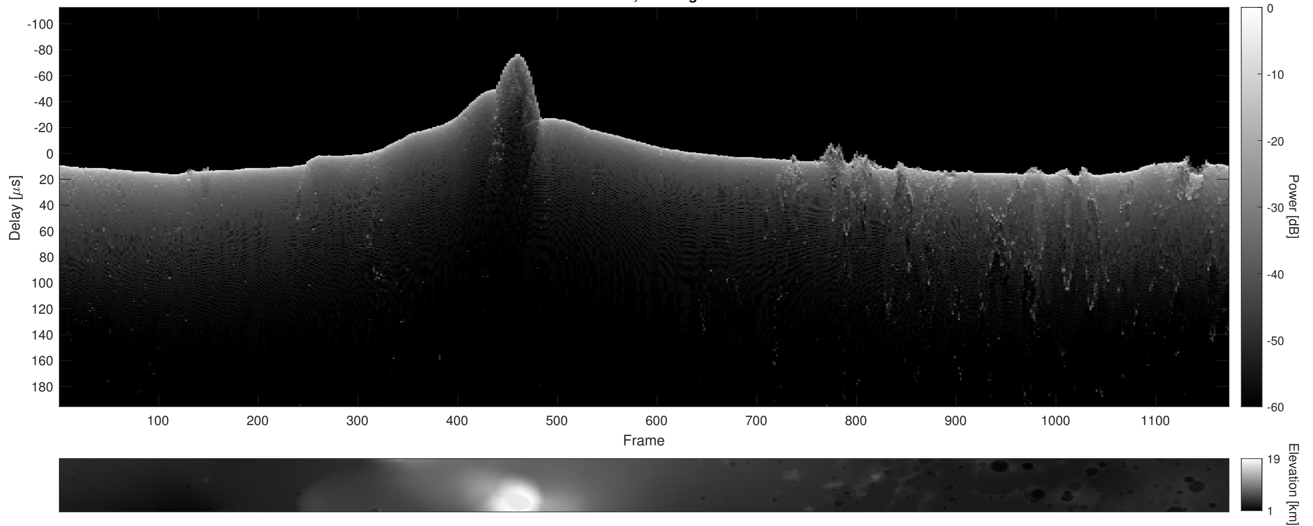
Orbit 9151, Cluttergram
