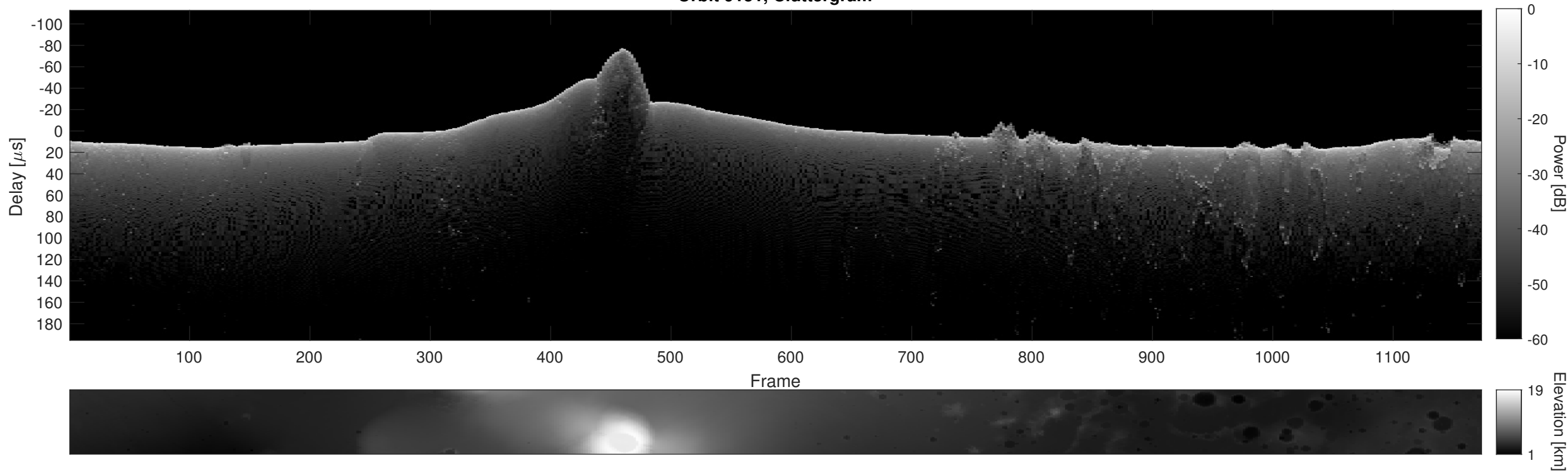
Orbit 9151, Cluttergram
