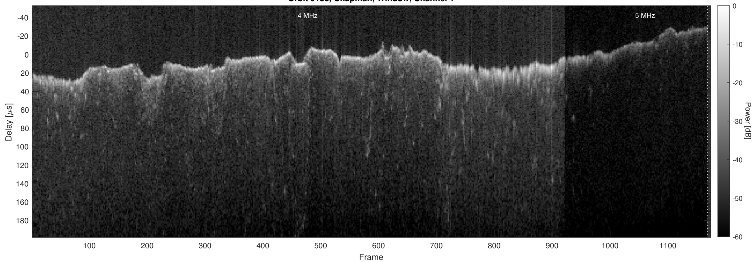
Orbit 9153, Chapman, Window, Channel 2
