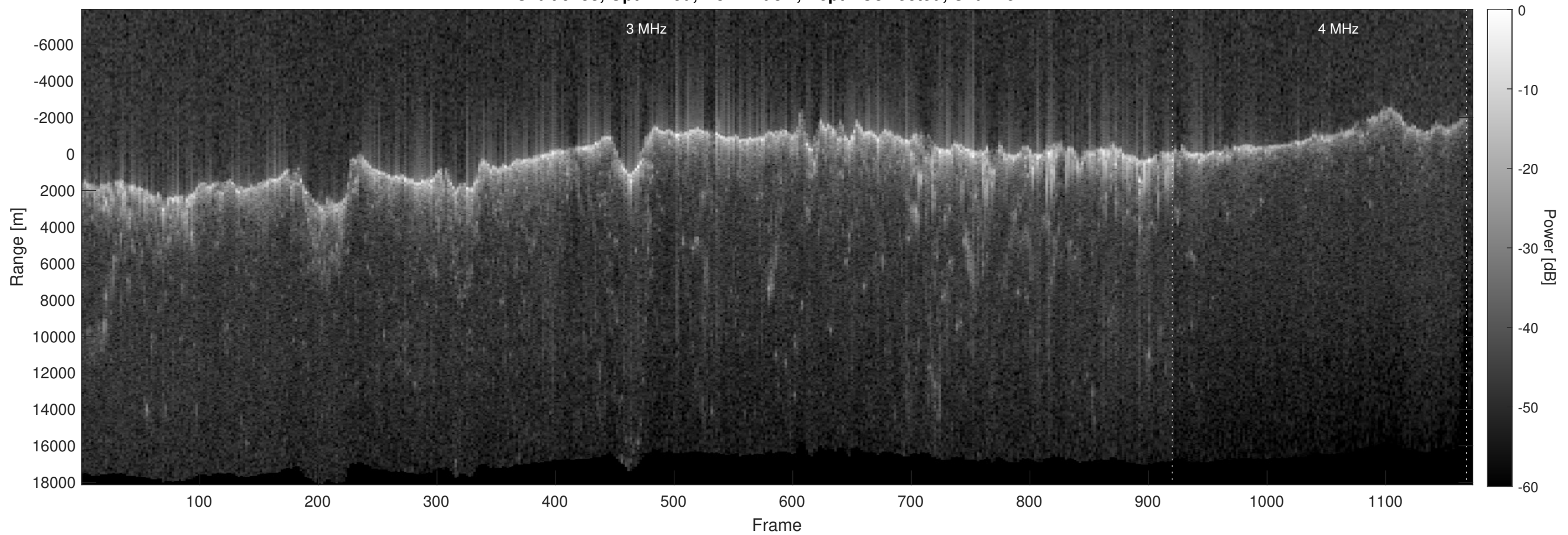
Orbit 9153, Optimized, No Window, Depth-Corrected, Channel 2
