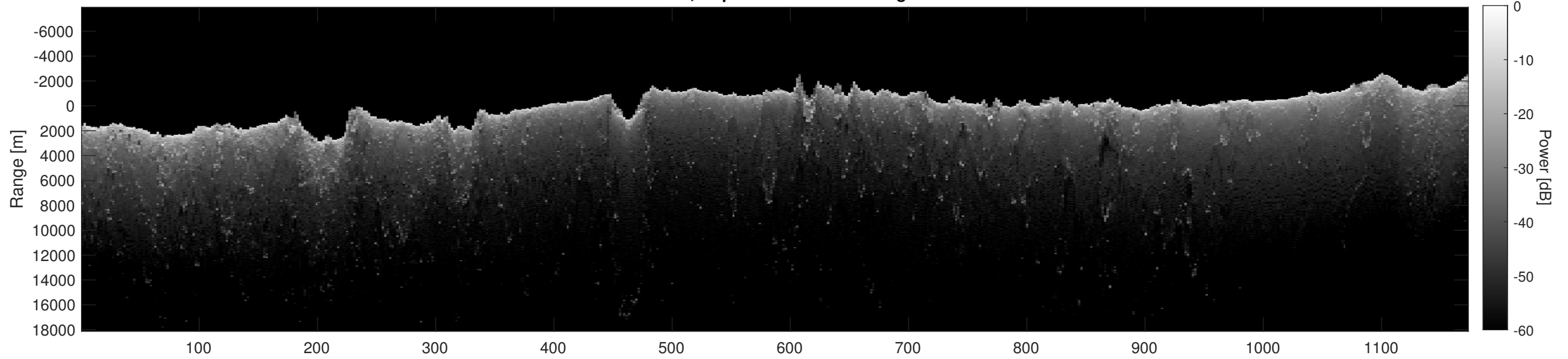
Orbit 9153, Depth-Corrected Cluttergram
