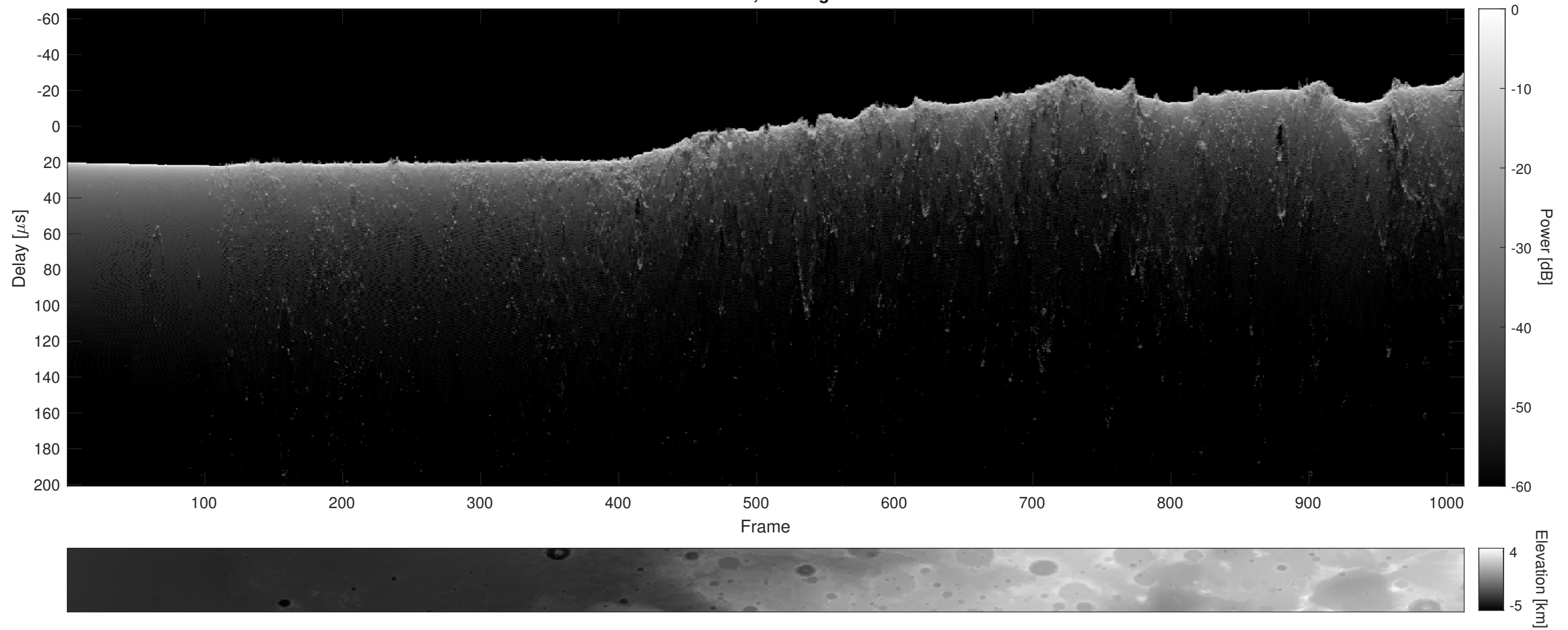
Orbit 9155, Cluttergram
