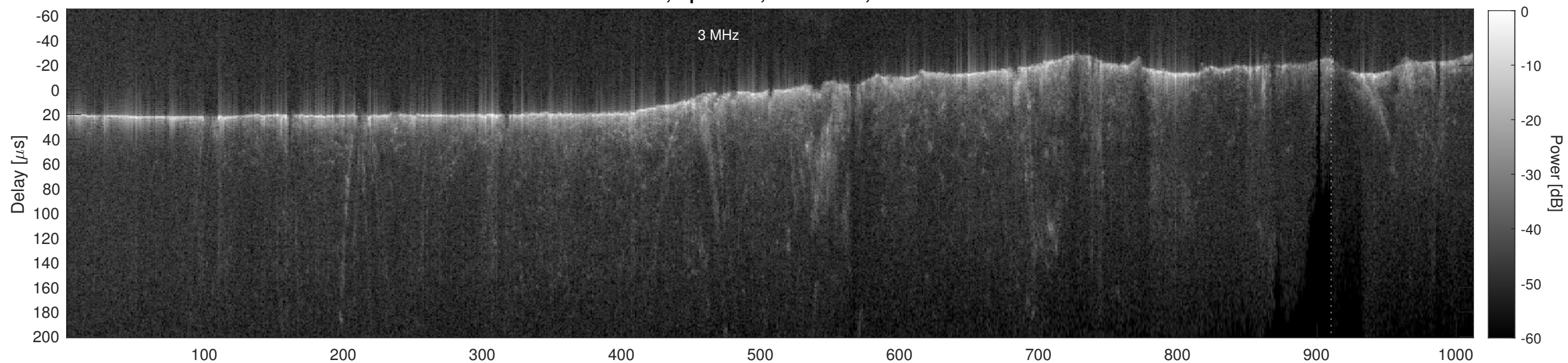
Orbit 9155, Cluttergram
