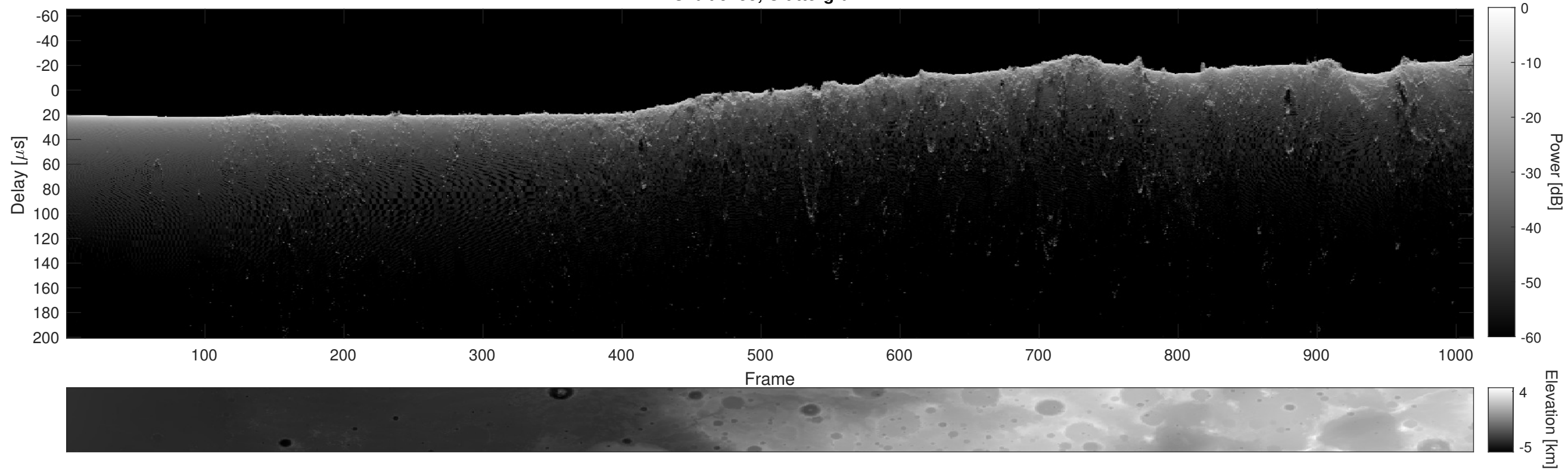
Orbit 9155, Cluttergram
