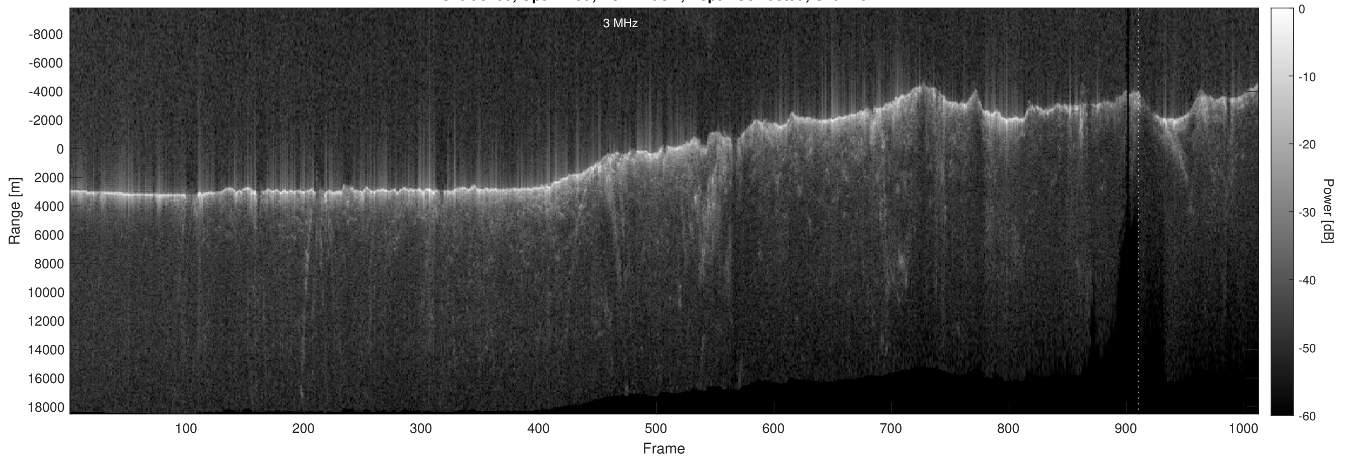
Orbit 9155, Optimized, No Window, Depth-Corrected, Channel 2
