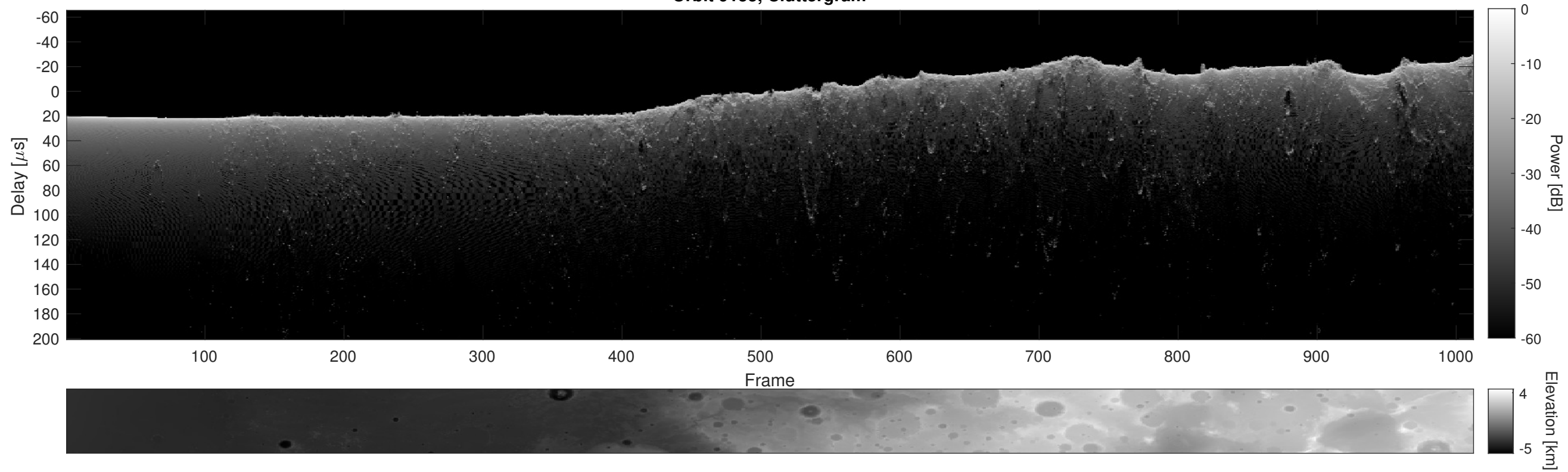
Orbit 9155, Cluttergram
