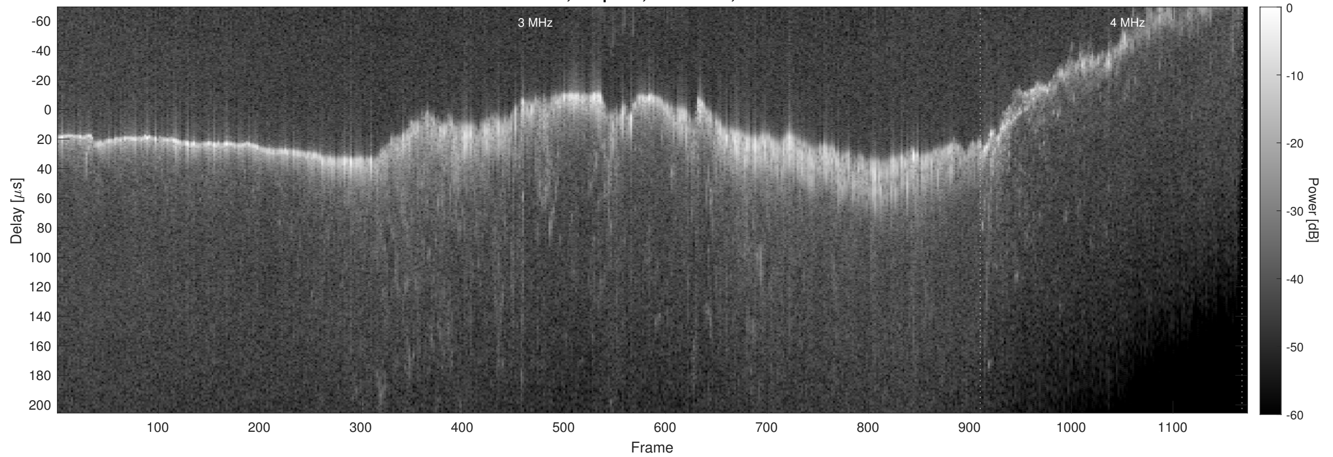
Orbit 9156, Chapman, No Window, Channel 2
