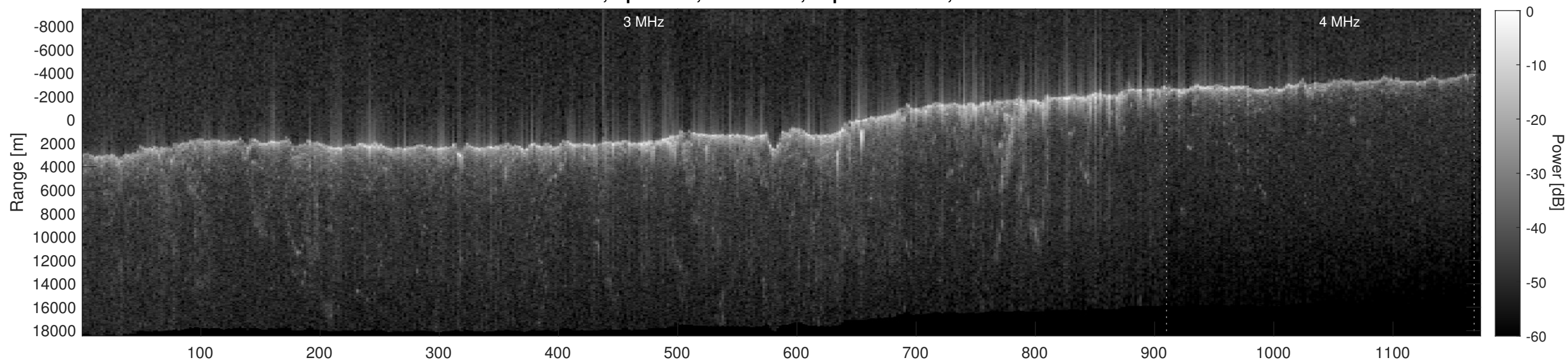
Orbit 9157, Depth-Corrected Cluttergram
