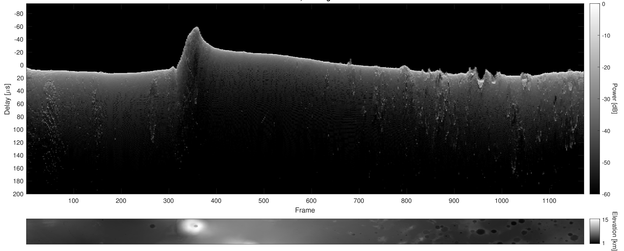
Orbit 9158, Cluttergram
