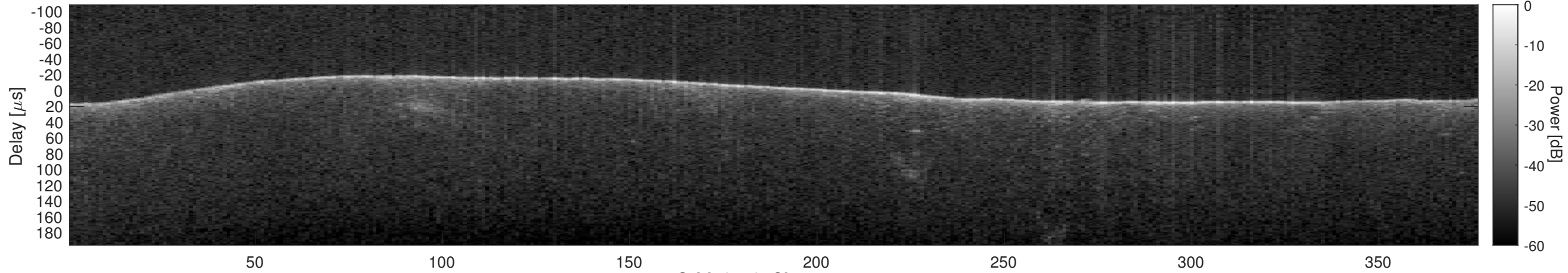
Orbit 9159, Cluttergram
