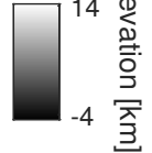
Elevation [km]
