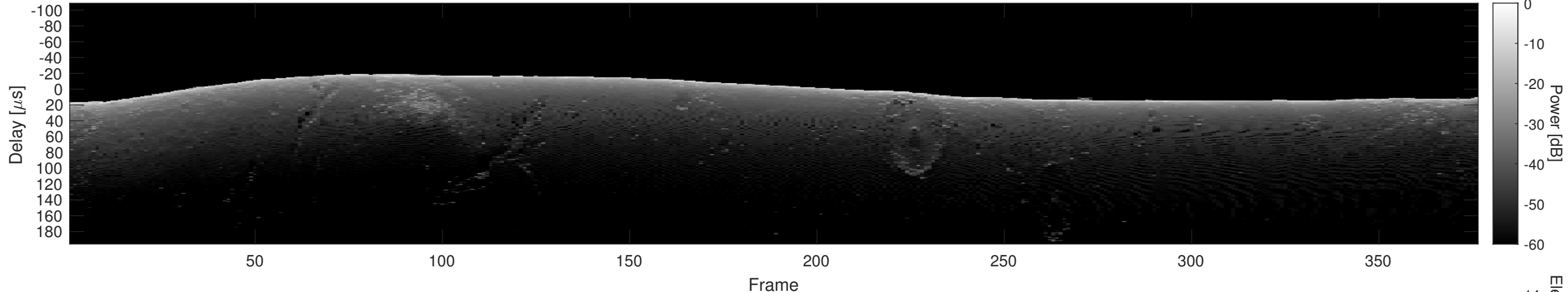
Orbit 9159, Cluttergram
