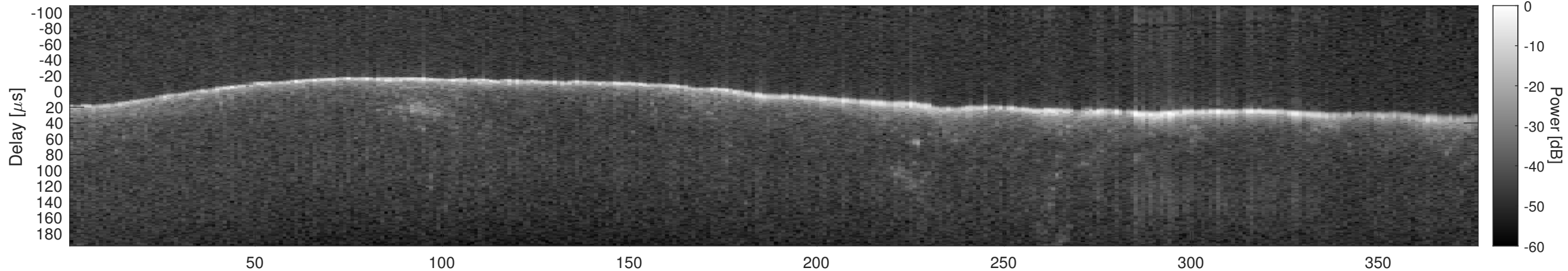
Orbit 9159, Window, Channel 2, Chapman
