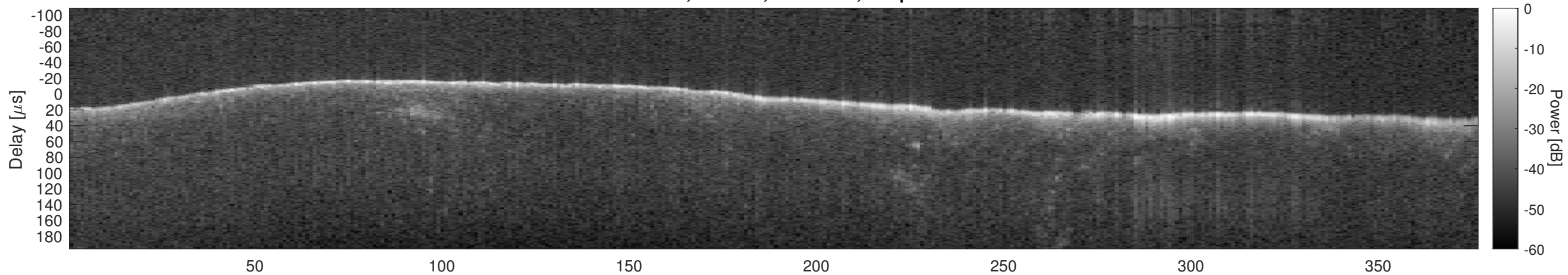
Orbit 9159, Window, Channel 2, Optimized
