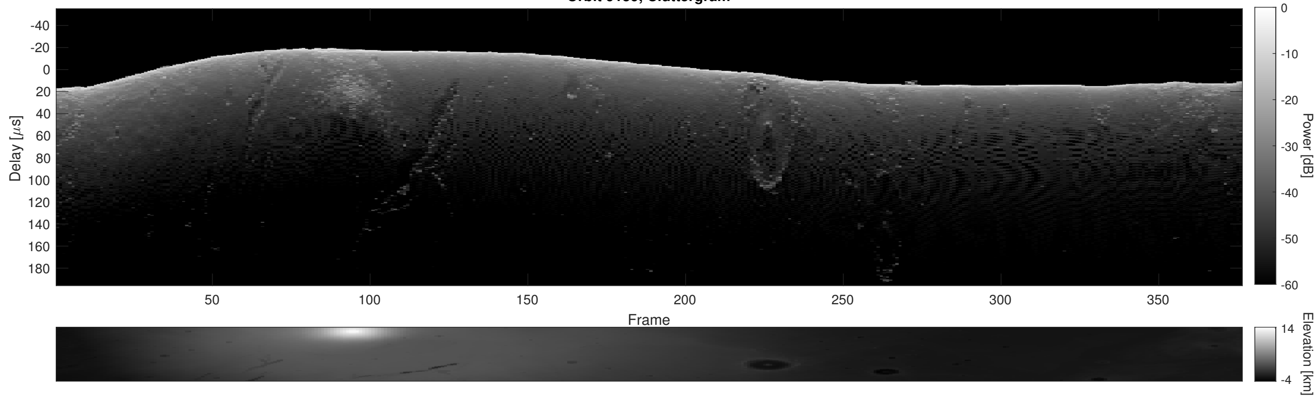
Orbit 9159, Cluttergram
