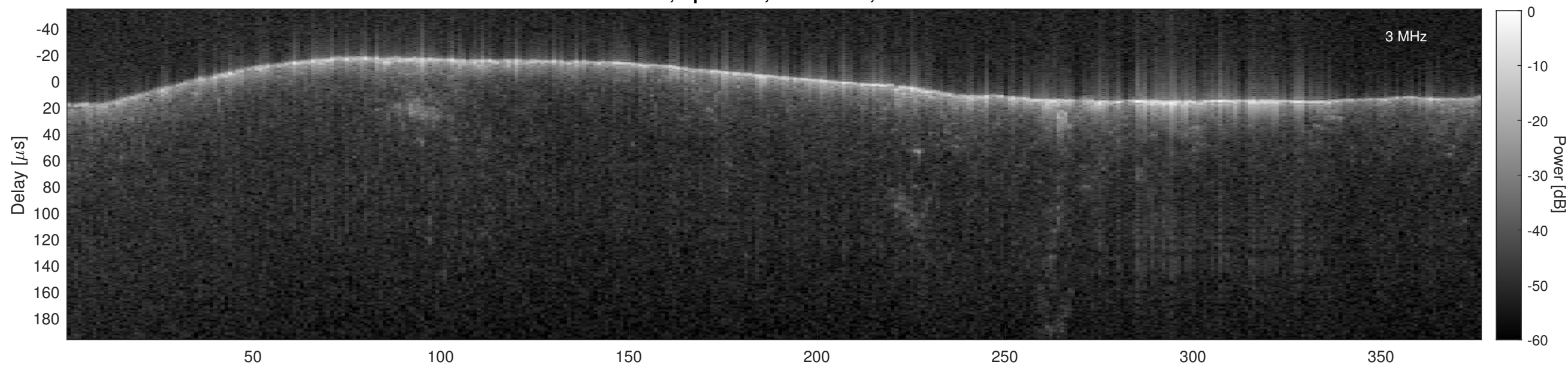
Orbit 9159, Cluttergram
