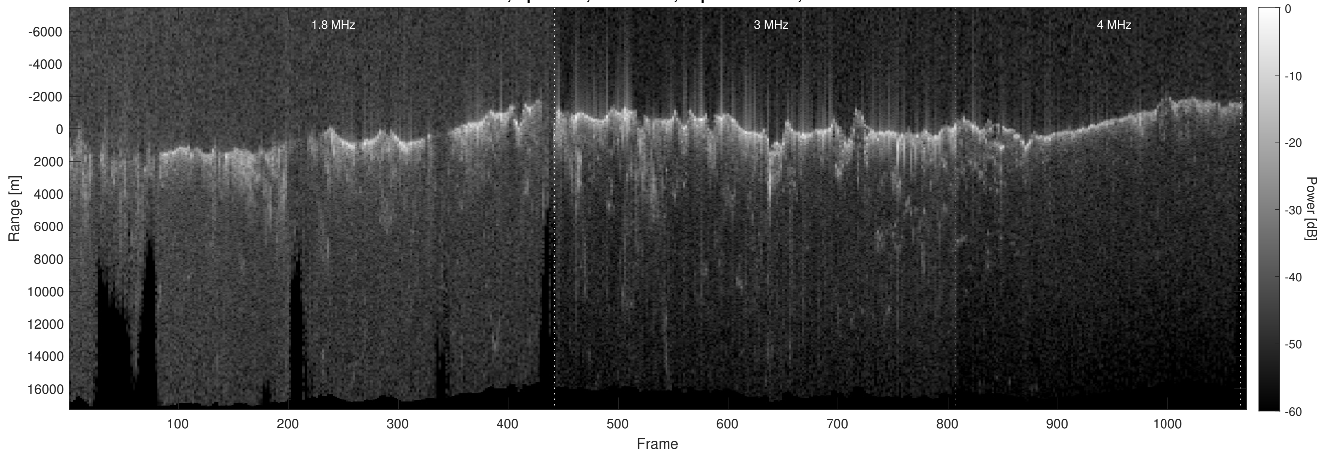
Orbit 9160, Optimized, No Window, Depth-Corrected, Channel 2
