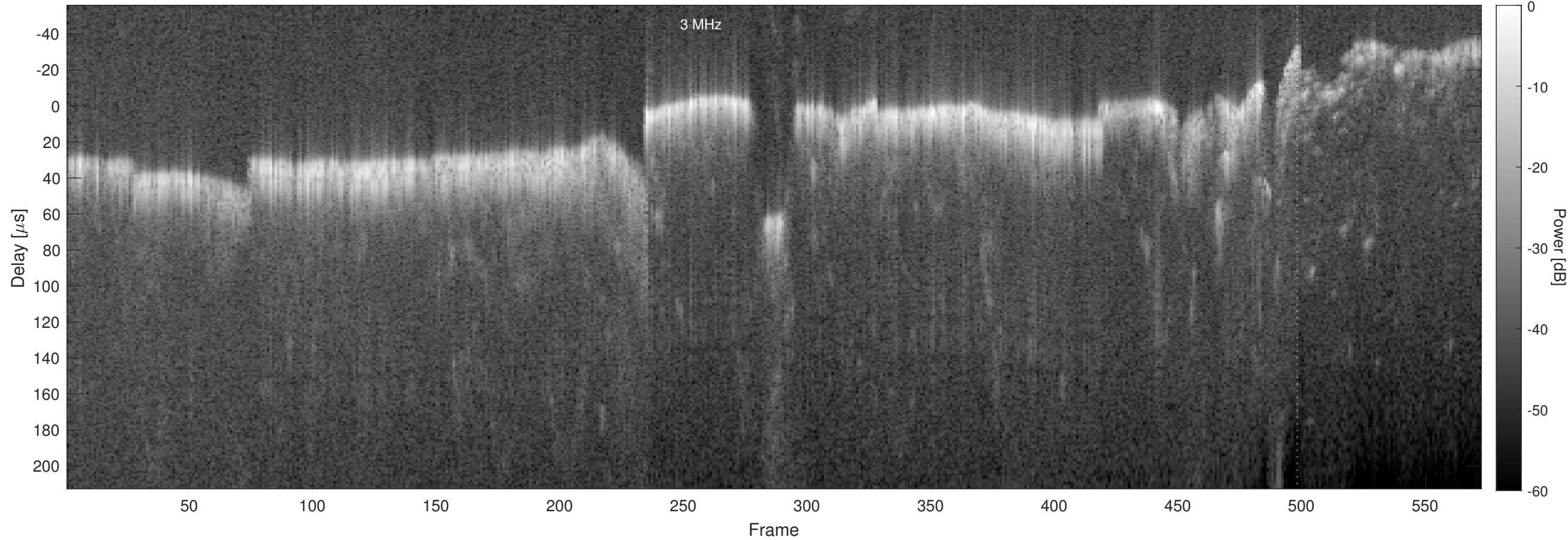
Orbit 9161, Chapman, No Window, Channel 2
