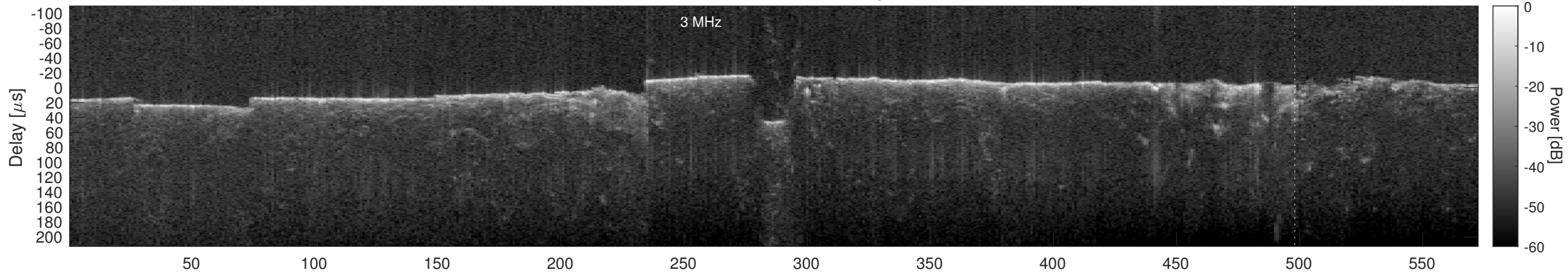
Orbit 9161, Cluttergram
