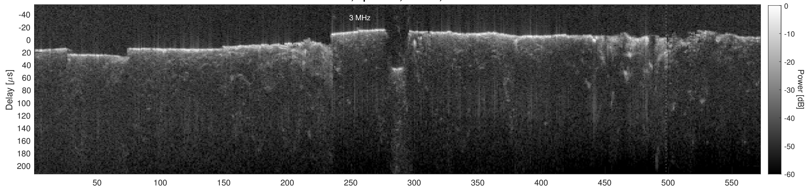
Orbit 9161, Cluttergram
