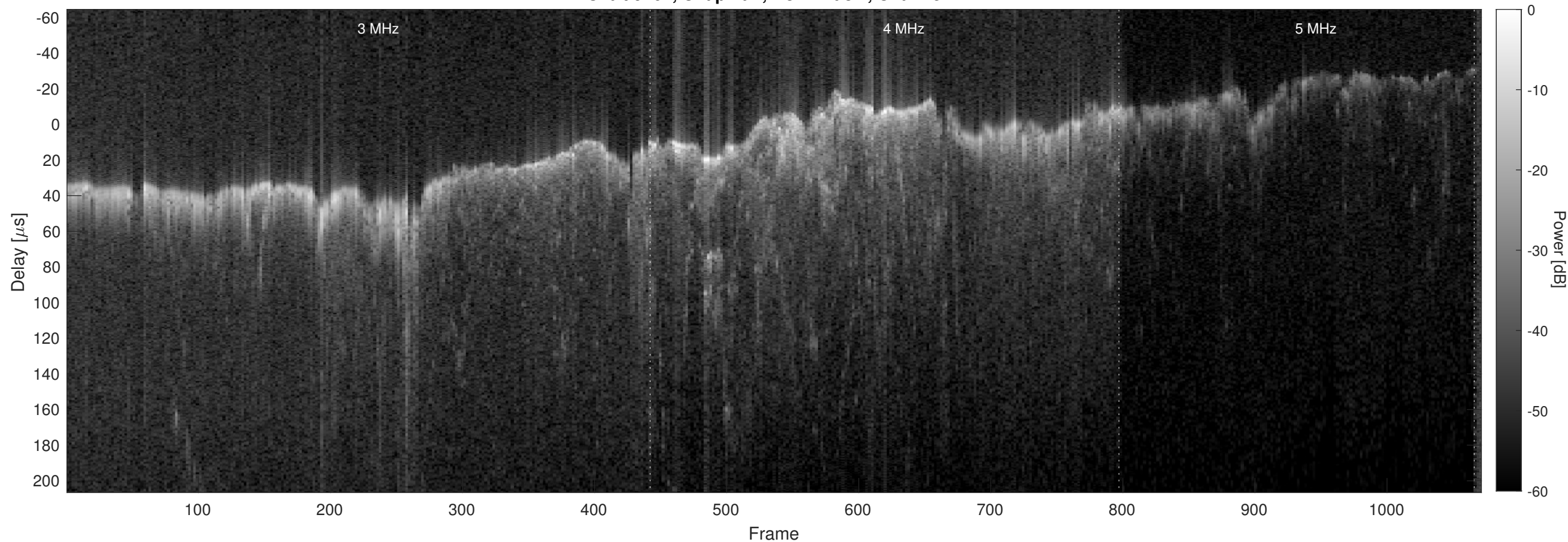
Orbit 9162, Chapman, No Window, Channel 2
