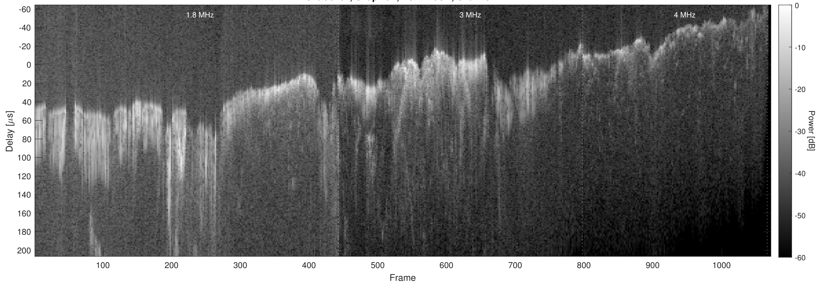
Orbit 9162, Chapman, No Window, Channel 2
