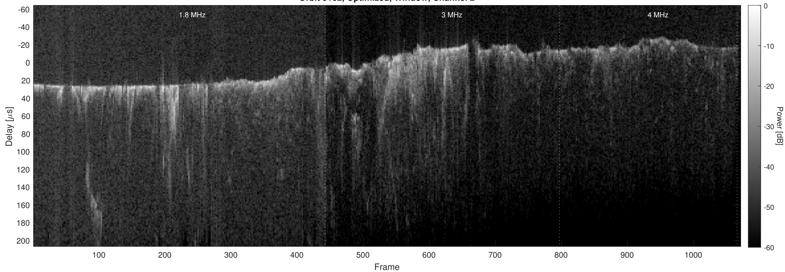
Orbit 9162, Optimized, Window, Channel 2
