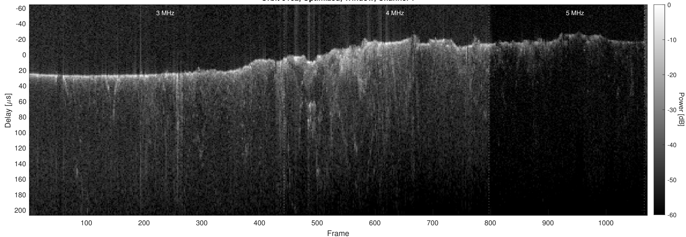
Orbit 9162, Optimized, Window, Channel 2
